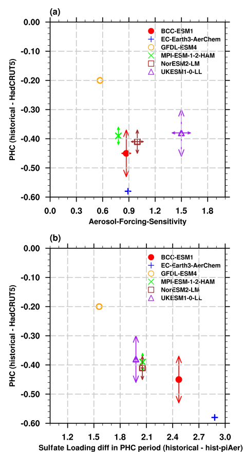
Figure 6. Pothole cooling (PHC) bias in ESMs (°C) versus (a) the aerosol forcing sensitivity ( \text{W mg}^{-1} ) and (b) sulfate loading differences ( \text{mg m}^{-2} ) during the PHC period. The arrows show the uncertainty ranges among the members in each ESM.
