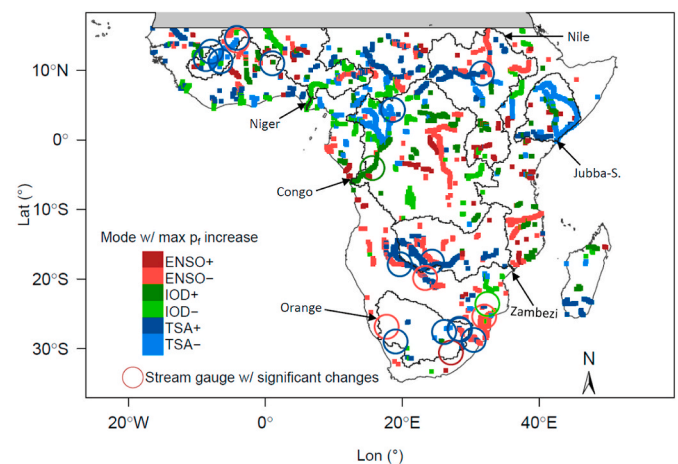
Fig. 3. Map of SSA highlighting the dominant climate mode (among positive and negative ENSO, IOD, TSA phases) for significant increase in flood hazard ( p_f > 25\% at a 95%-confidence level) for all river cells from the streamflow reanalysis and 21 stream gauges (out of 48 with sufficiently long records) where significant increases in 5-year return level flood probability are found (circle dots). The boundaries of the six major SSA river basins are drawn (black line) with labels indicating the river basin name.
