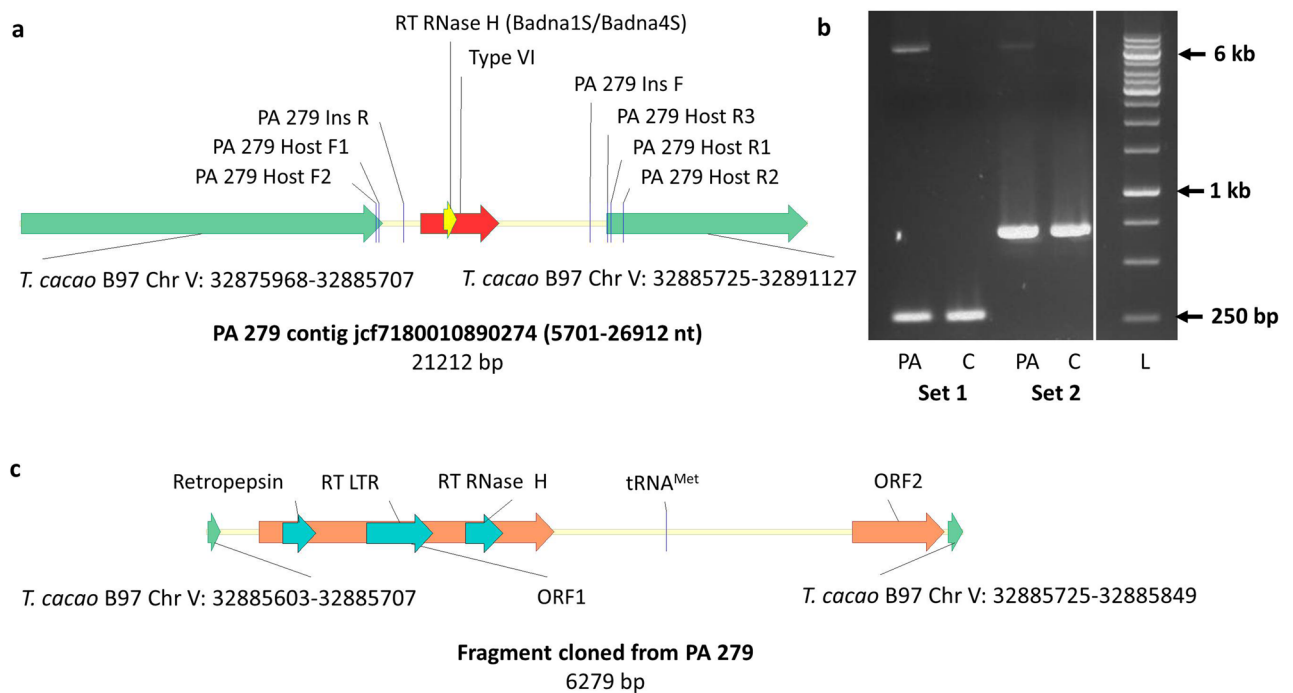
Figure 4. Amplification of type VI viral insertion from cacao clone PA 279. (a) Alignment of PA 279 contig jcf7180010890274 and B97 T. cacao genome Chromosome V. Green arrows represent genomic region of cacao clone B97 bordering 6050 bp of type VI viral insertion. Vertical lines indicate location of primers including primer set 1 (PA 279 Host F1, PA 279 Host R1) and set 2 (PA 279 Host F2, PA 279 Host R2) used to amplify the viral insert along with the bordering host sequence, and primers used in the multiplex assay to screen cacao germplasm for viral insertion type VI (PA 279 Host F1, PA 279 Ins R, PA 279 Ins F and PA 279 Host R3). (b) Amplification of the viral insert along with the bordering host sequence from PA 279 (PA) and Criollo 11 (C) clones. The 243 and 635 bp fragments amplified in both clones with primer set 1 and set 2 represent virus- allele (lacking viral insertion) whereas a fragment between 6 to 7 kb amplified in PA 279 clone in both primer sets represents virus + allele. (c) Open reading frames (brown arrows) and conserved domains (light blue arrows) present in the fragment amplified from PA 279 clone harbouring host genome and type VI viral sequence. Full-length gel of section (b) is presented in Supplementary Fig. 1.
