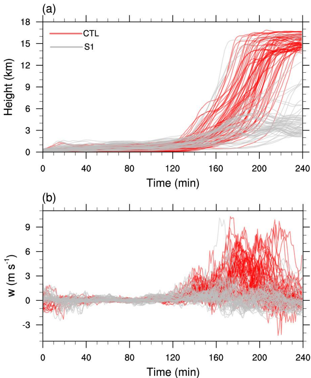
948 949 Fig. 11. The evolution of (a) parcel height (km) and (b) vertical velocity ( \text{m s}^{-1} ) along the 4-h 950 trajectory for the top 20% of the parcels that are stratified by their maximum height of the 4-h 951 trajectory. The red and gray lines denote the trajectories in CTL and S1, respectively.
