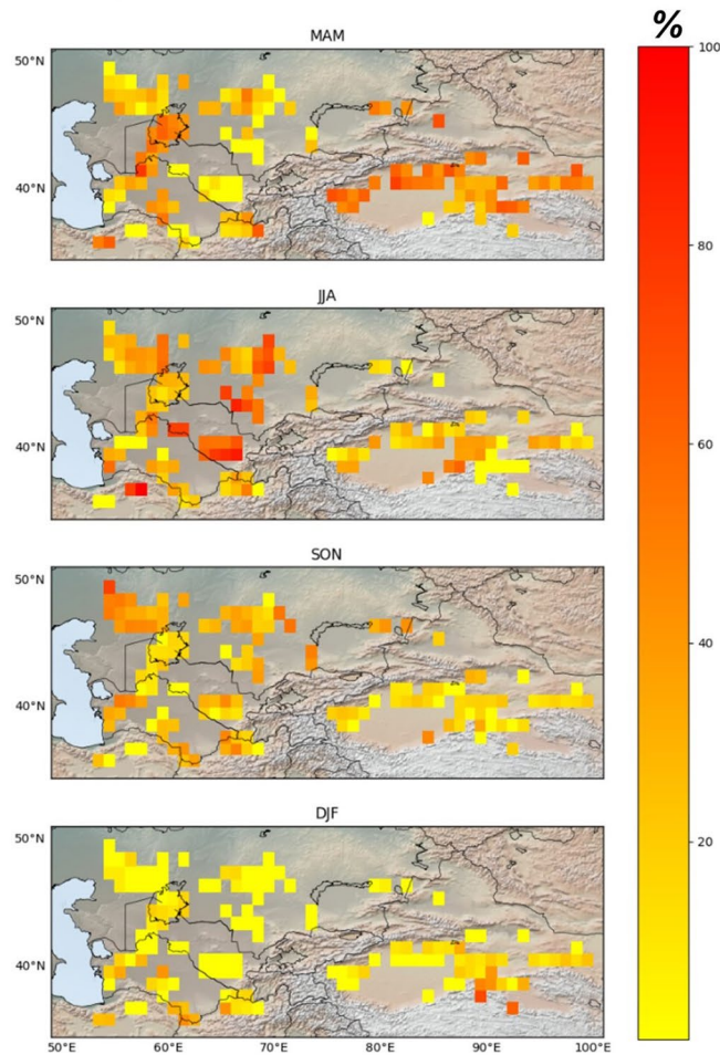
Figure 4. Mean seasonal statistics of DSA averaged over the 2003–2012 period. Grid cells with less than one dusty day per year are transparent. DSA, dust source activation.
