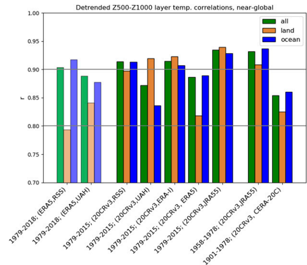
FIG. 15. Correlations between near-global (70°S–82°N) detrended 500–1000-hPa layer temperatures \bar{T} for the given time periods and land/sea masks. Correlations between ERA5, RSS, and UAH are shown on the left in lighter colors for clarity.
