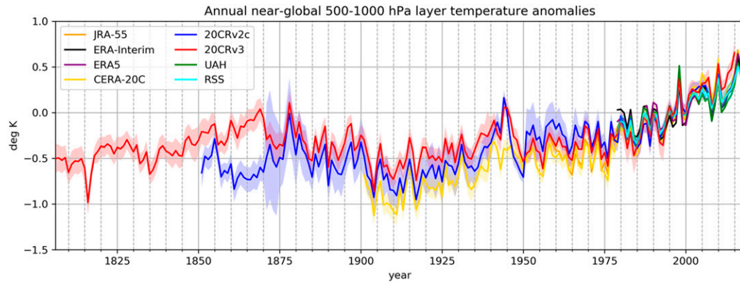
FIG. 14. Near-global (70°S to 82°N) average 500–1000-hPa layer temperature \bar{T} anomalies with respect to each dataset's 1981–2010 climatology, estimated from geopotential heights in all reanalyses. The confidence intervals are calculated as twice the ensemble standard deviation and shown for 20CRv2c, 20CRv3, CERA-20C, and RSS; see text for description of issues in 20CRv2c uncertainty. UAH and RSS temperature in the lower-troposphere products were each regressed onto ERA5 for the available 1979–2018 period.
