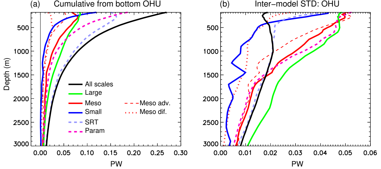
Figure 5: (a) Integrated horizontally and from the bottom to each depth OHU (i.e., increase in downward heat transport in 1pctCO2 from piControl across each depth) due to all scales (“All scales”) and its partitioning into contributions from the resolved circulation (“Large”), all mesoscale and submesoscale eddy-related processes (“Meso”) and all diapycnal and other effects (“Small”). Also shown are the contributions from the super-residual transport (SRT = Large+Meso) and all parameterized (in these AOGCMs) processes (Param = Small+Meso), as well as the partitioning of Meso into contributions from eddy advection (Meso adv.) and diffusion (Meso dif.); (b) Inter-model standard deviations (STDs) corresponding to the curves in panel (a).
