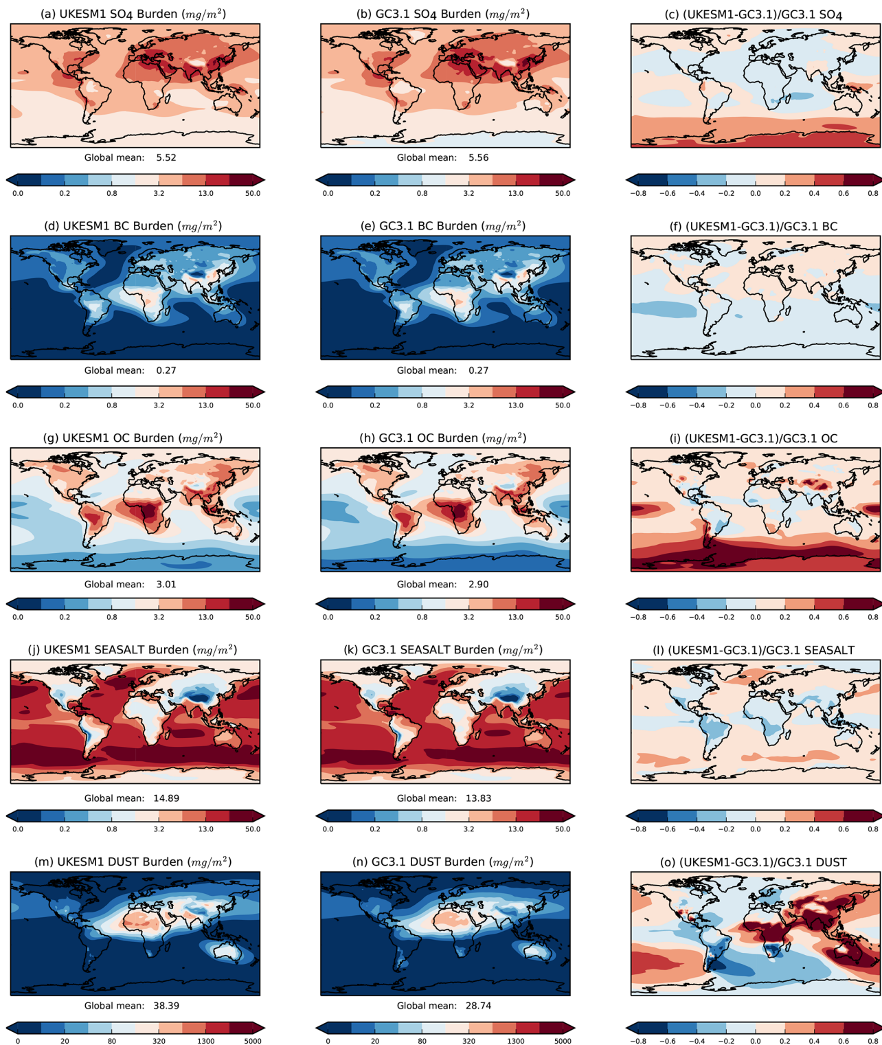
Figure 3. Annual mean burden (mg m -2 ) of SO 4 , BC, OC, sea salt and mineral dust aerosol in (left column) UKESM1, (middle column) GC3.1 and (right column) their fractional difference. The annual mean burdens are computed from the nine- and four-member historical ensemble means from UKESM1 and GC3.1, respectively, from 1980 to 2014 inclusive. Note the different contour levels in panels (m) and (n).
