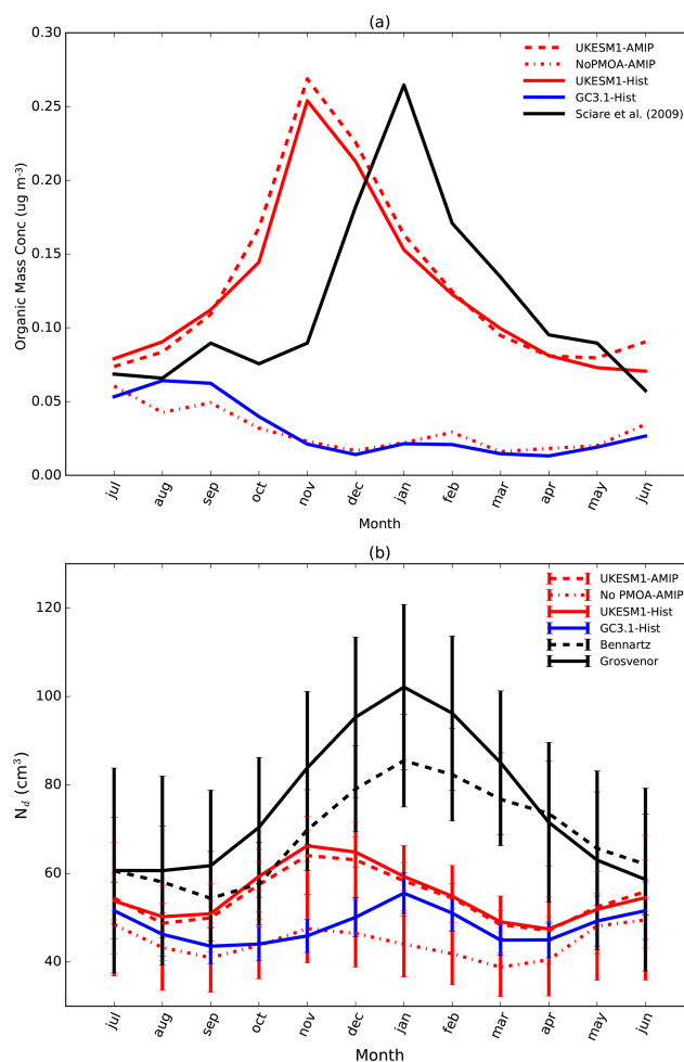
Figure 16. Seasonal evaluation of simulated (a) OM surface mass concentration at Amsterdam Island and (b) N_d averaged over 30\text{--}70^\circ \text{S} from UKESM1-AMIP, a UKESM1-AMIP simulation with no PMOA source and the UKESM1 and GC3.1 historical ensemble means. The OM mass observations in panel (a) are taken from Sciare et al. (2009). The N_d observations used in panel (b) are taken from the Grosvenor et al. (2018b) and Bennartz and Rausch (2017) satellite N_d products. The simulated monthly N_d data are taken from 2003 to 2014 inclusive to match the satellite temporal coverage. Given the low data coverage of satellite retrievals in the austral winter, the model and Bennartz data have been spatially sampled according to the Grosvenor data product.
