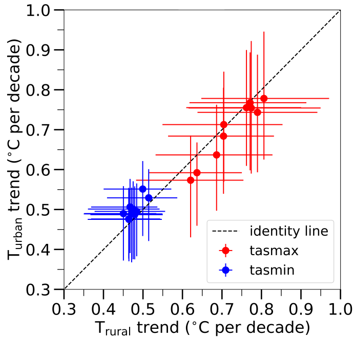
FIG. 2. Comparison of trends of urban and rural temperatures (in ^{\circ}\text{C} per decade) over summers (June-July-August) in 1981–2079. Each dot represents one studied city. The error bars indicate the 12-member ensemble spread of UKCP18-regional. Red dots show trends in summer daily maximum temperature, whereas blue dots show trends in summer daily minimum temperature. The dashed line shows the identity line.
