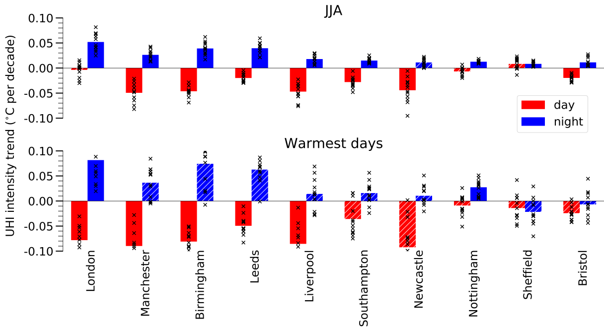
FIG. 4. UHI intensity trends (in ^{\circ}\text{C} per decade) in 1981–2079 for daytime (red) and night-time (blue) near-surface air temperatures. The bars show the UKCP18-regional ensemble-mean values whereas the crosses indicate individual ensemble members. Bars where the 12-member ensemble range crosses zero are hatched. The upper panel shows trends in summer (June-July-August), whereas the bottom panel shows trends in UHI intensities on annual three consecutive warmest days.
