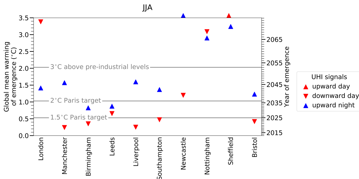
FIG. 6. Global mean warming of emergence of summer daytime (red) and night-time (blue) UHI signals in the 10 most populous cities in England. Upward triangles indicate positive (upward) signals, whereas downward triangles indicate negative (downward) signals. Warming of emergence is measured in global mean warming in °C since 2008–2018. The right vertical axis shows the corresponding year of emergence based on the ensemble mean of the UKCP18-global simulations. The grey horizontal lines indicate the Paris Agreement temperature targets and 3°C global warming above pre-industrial levels (1850–1900), based on the UKCP18-global simulations and global mean warming between 1850–1900 and 2008–2018 in HadCRUT4-CW. Triangles on top of the figure indicate daytime (red) and night-time (blue) UHI changes that do not emerge in the UKCP18 simulations.
