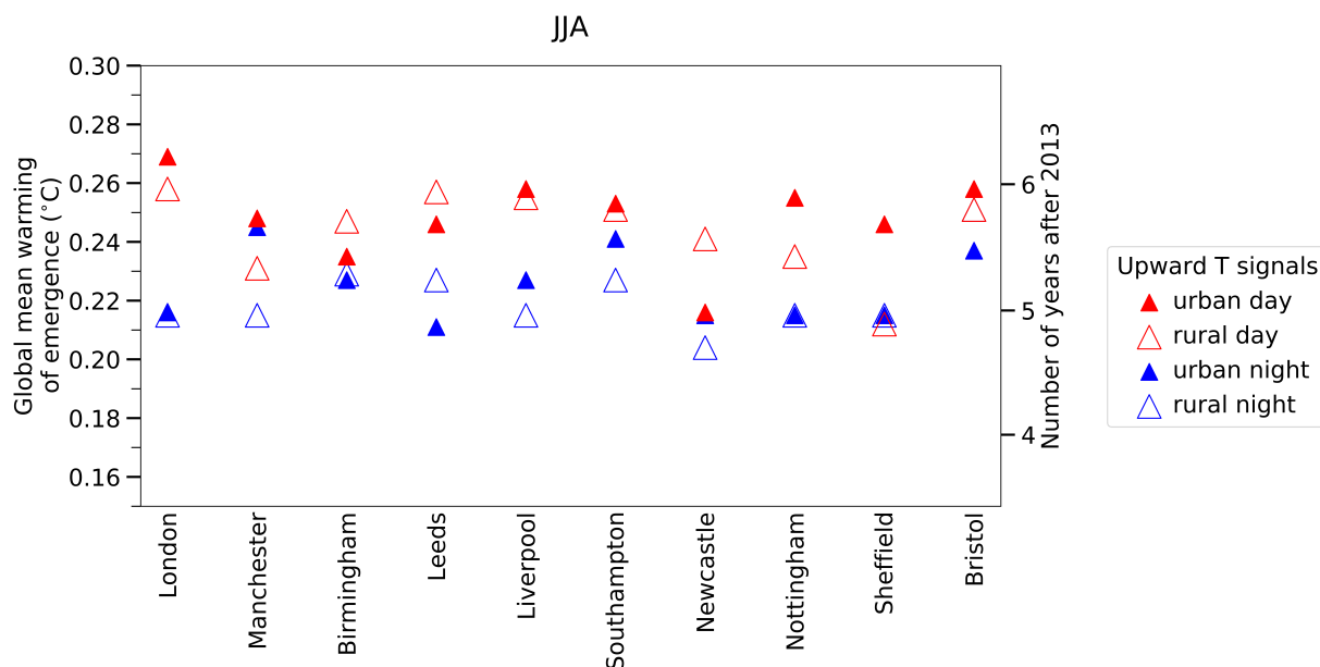
FIG. 5. Global mean warming of emergence of summer daytime (red) and night-time (blue) urban (filled triangles) and rural (empty triangles) temperature signals in and around the 10 most populous cities in England. All signals are positive as indicated by the upward triangles. Warming of emergence is measured in global mean warming in °C since 2008–2018. The right vertical axis shows the corresponding number of years after 2013 (the middle year of the 2008–2018 baseline), based on the ensemble mean of the UKCP18-global simulations. 1.5°C global warming above pre-industrial levels corresponds to 0.53°C warming since the average of 2008–2018, which is above the vertical scale of this figure.
