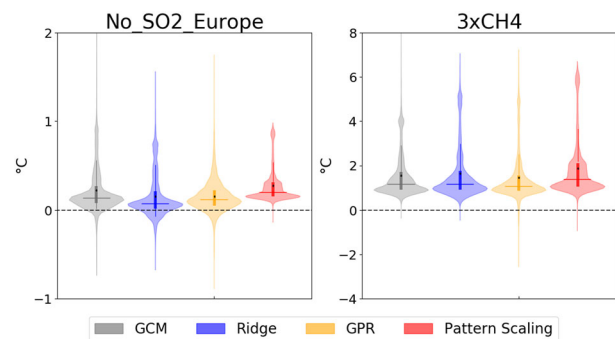
Fig. 2 Distribution of predicted grid-point scale surface temperature responses in °C for all methods for one short-lived forcing, No_SO 2 _Europe, and one long-lived forcing, 3xCH 4 . The central vertical boxes indicate the interquartile range shown on a standard box plot, the horizontal line shows the median and the black point shows the mean. The horizontal width shows the distribution of temperature values overall grid points, i.e. the wider regions highlight that more grid points have this value of predicted temperature response. Note the different vertical scales.
