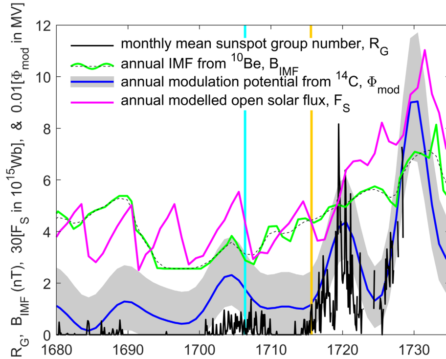
Fig. 16. The emergence of the solar activity from the MM in the “recovery phase”. The black line gives the monthly means, R_G , of daily group sunspot numbers by Vaquero et al. (2016): note that values are only given for months in which more than 15 days of observations were available. The green line shows monthly mean of the near-Earth interplanetary magnetic field, B_{IMF} , derived by McCracken & Beer (2015) from the ^{10}\text{Be} cosmogenic isotope abundances from the Dye-3 ice-core and North Greenland Ice Core Project (NGRIP), both from Greenland (Beer et al., 1998; Berggren et al., 2009): the black dashed line is the same data passed through a 1-4-6-4-1 filter. The blue line gives annual means of the heliospheric modulation potential, \Phi_{mod} , derived from both the ^{14}\text{C} and ^{10}\text{Be} cosmogenic isotopes: the surrounding area gives the 2-sigma uncertainty band (Muscheler et al., 2007). The mauve line is the open solar flux, F_S , modelled by Lockwood & Owens (2014) from sunspot numbers. The vertical cyan and orange lines mark the times of the 1706 and 1715 eclipses, respectively.
