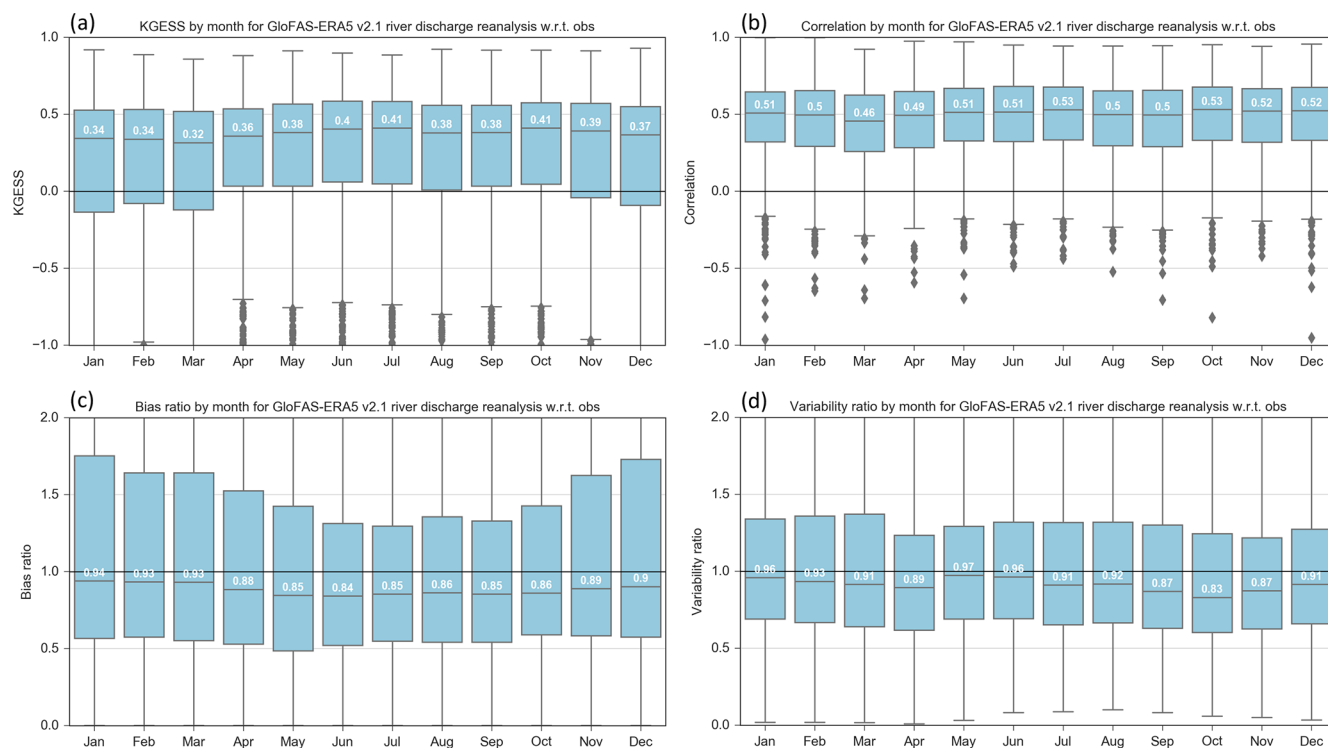
Figure 8. Performance metrics for each month for all 1801 stations. Modified Kling–Gupta efficiency skill score (KGESS) (a) with decomposition of \text{KGE}' into Pearson correlation (b), bias ratio (c), and variability ratio (d). Boxes represent the IQR and horizontal grey line the median. Whiskers extend to the most extreme data point unless the data point is more than 1.5 times the IQR from the box and is instead represented as an outlier (grey diamond).
