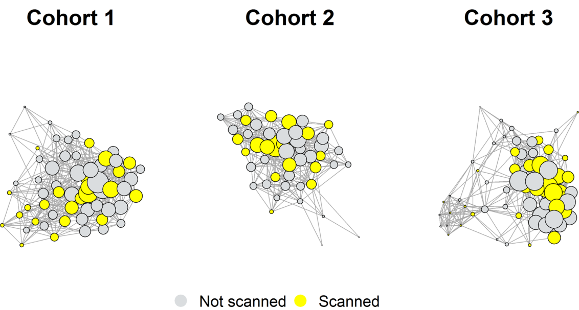
Figure 1. Social networks of cohorts 1, 2 and 3, depicting reciprocal friendships. Nodes represent students; lines (edges) represent mutually reported social ties where students rated the amount of time they spent with each other as “more than some” or “most” of the time. fMRI cohorts are depicted in yellow; students who provided information about their social interactions but were not included in the fMRI cohort are shown in grey. The size of each node depicts the Eigenvector centrality of that student. Eigenvector centrality is a measure of the relative importance/influence of a node in the network. Nodes with high importance (those who are themselves well-connected and are connected to others who are well-connected) have higher centrality (these are the largest nodes in the network), those with low importance have low centrality (these are the smallest nodes in the network).
