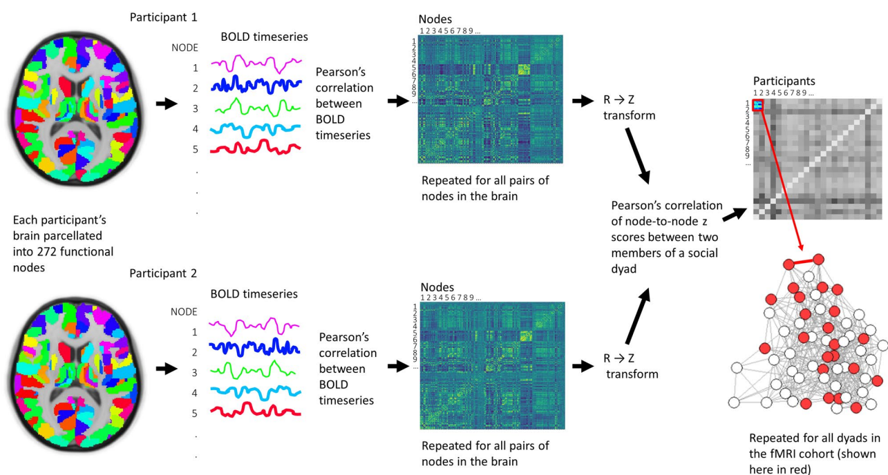
Figure 3. Processing pipeline for determining similarity of resting-state functional connectivity between participants. Mean blood oxygen level-dependent (BOLD) time series data for each brain parcel were correlated within participants and then whole-brain correlation matrices were compared between participants.
