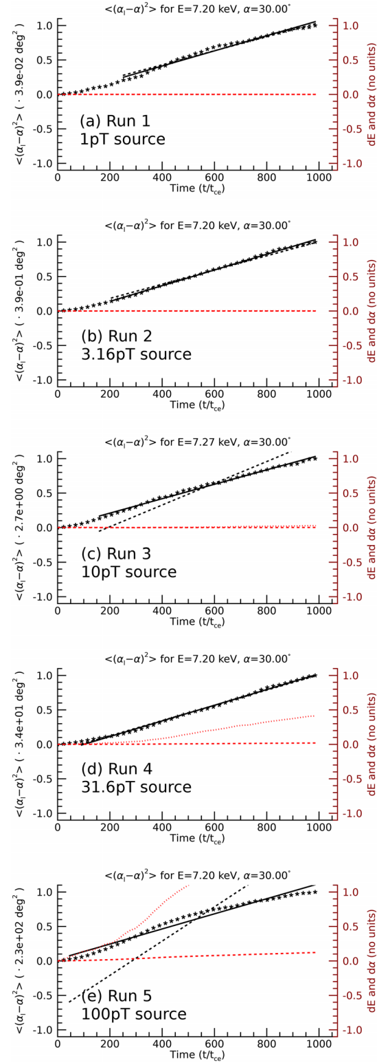
Figure 2. Evolution of \langle(\alpha_l - \alpha)^2\rangle for all five runs (asterisks) for electrons initially in a given bin ( E, \alpha ) \approx (7 keV, 30^\circ ). The solid black line is a linear fit applied to the data over (a) 250t_{ce} < t < T ; (b) 200t_{ce} < t < T ; (c) 150t_{ce} < t < T ; (d) 100t_{ce} < t < T ; (e) 50t_{ce} < t < T ( T \approx 1,008t_{ce} for all plots). The gradient of the dashed black line corresponds to the evolution of \langle(\alpha_l - \alpha)^2\rangle as predicted using the PADIE code. The dashed red line is the evolution of \langle\Delta E\rangle , and the dotted red line is the evolution of \langle\Delta\alpha\rangle . Black and red quantities are defined by the left-hand and right-hand axes, respectively. The left-hand y-axes have scales as defined by the quantity in brackets and are formally in units of \text{deg}^2 .
