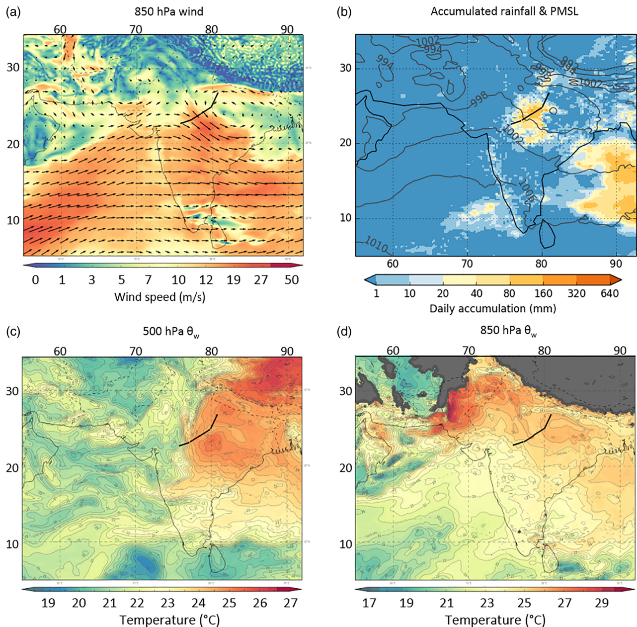
FIGURE 15 Analysis at 0600 UTC (11:30 local) on July 7, 2016 of (a) winds at 850 hPa, (c,d) \theta_w at 500 and 850 hPa, respectively, and (b) PMSL and observed accumulated rainfall (as in Figure 12f), with the planned flight track overlaid in solid black lines
