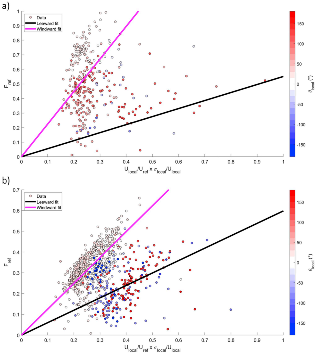
Fig. 9. As Fig. 7, but with \left(\frac{U_{\text{local}}}{U_{\text{ref}}} \times \frac{\sigma_{\text{local}}}{U_{\text{local}}}\right) .
