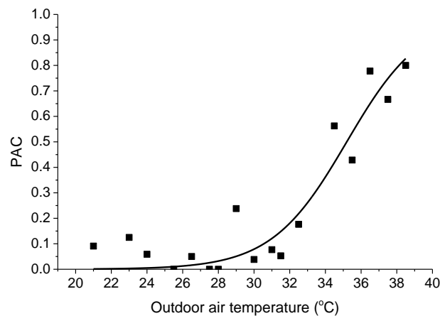
Figure 8. Proportion of air-conditioned rooms as a function of outdoor air temperature in residential buildings
