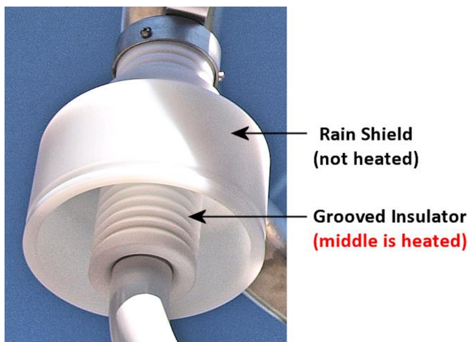
Fig 15.15. Electrical isolation method for the sensing electrode of a Biral BTD-300 thunderstorm detector, showing the shielded and heated PTFE insulator to prevent water-induced grounding during all weather conditions. (Photo: A.J. Bennett)
