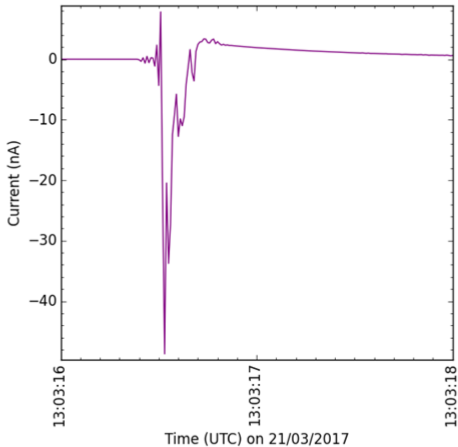
Fig 15.11. Displacement current induced on the electrode of a BTD-300 thunderstorm detector by a lightning flash approximately 20 km away.
