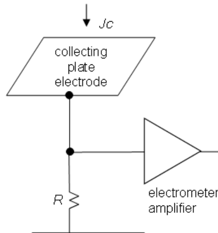
Fig 15.8. Concept of a plate electrode measurement for the vertical conduction current density. A horizontal plate is positioned slightly above the earth's surface on insulators, and the current flowing from it to the earth's surface measured.
