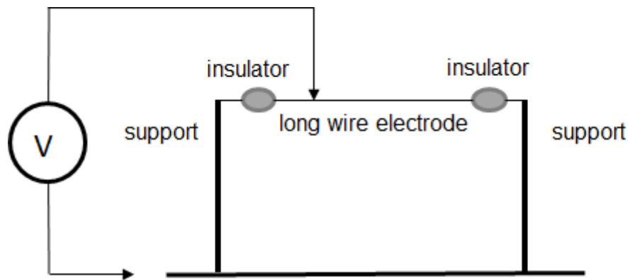
Fig 15.4. Passive wire antenna. A length of uninsulated wire is stretched between two support masts, using good quality insulators. The potential on the wire is measured using an electrometer voltmeter. (Typical dimensions: length of long wire 20m, support mast height 1m).
