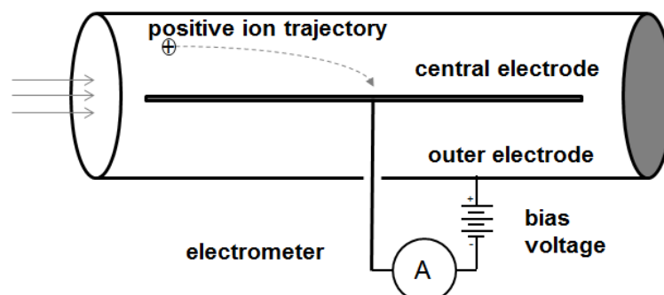
Fig 15.6. Concept of the operation of a cylindrical ion collector, with the outer electrode grounded. A bias voltage is used to establish a radial electric field. Ion-laden air is driven through the system, and ions are deflected by the electric field and collected at the central electrode, and the integrated current measured.
