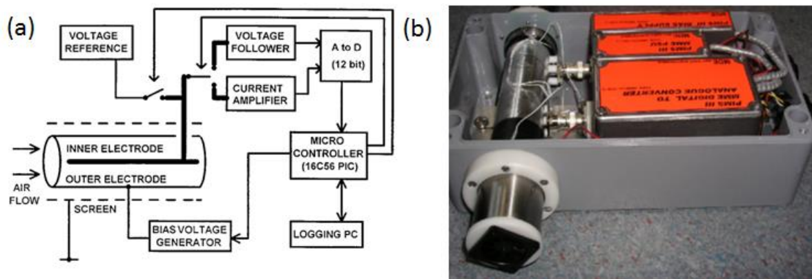
Fig 15.7. Programmable Ion Mobility Spectrometer (PIMS) of [15.72] shown in block diagram form (a), and physically (b). In (b), the fan providing the forced ventilation is at the foreground end of the cylindrical sampling electrodes on the left. ((a) from AIP, (b) Photo: R.G. Harrison).
