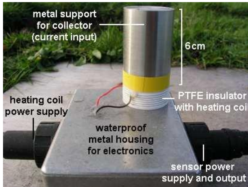
Fig 15.14. Heated PTFE insulation of the Geometrical Displacement and Conduction Current Sensor (GDACCS). Ultra-high quality insulation is required continuously between the sensing electrode and ground. (From [15.46])
