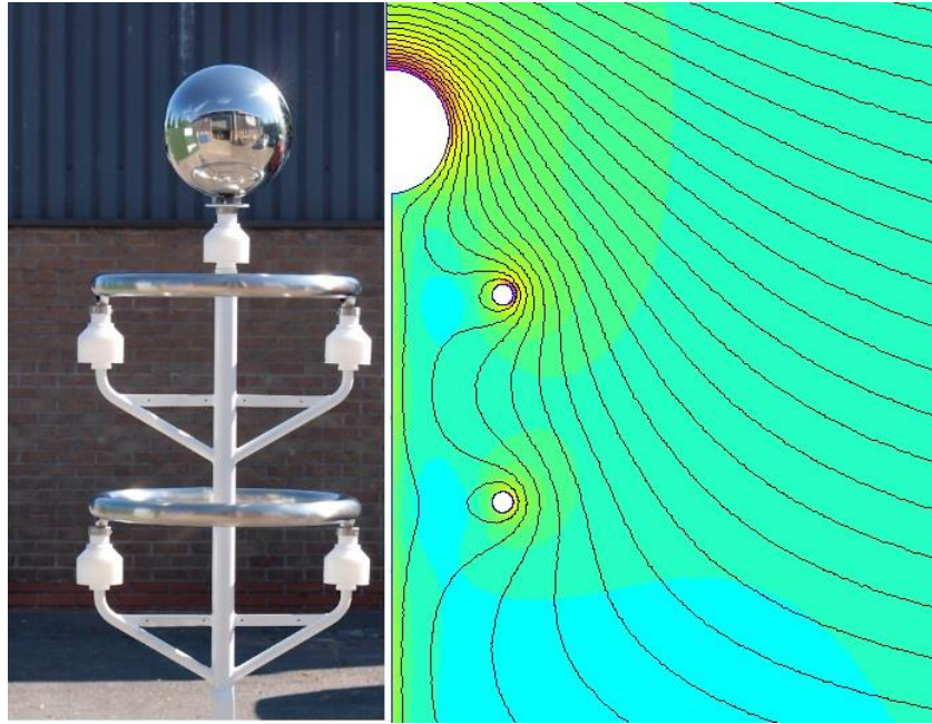
Fig 15.12 The Biral BTD-300 thunderstorm detector, with modelled lines of equipotential (black) compared to ground and electric field magnitude (colours) surrounding the three stainless-steel sensing electrodes. Warmer colours denote stronger field. (Photo and model: A. J. Bennett).
