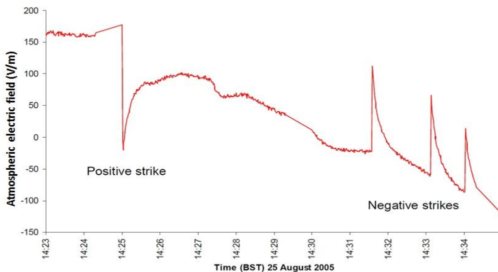
Fig 15.3 Electrostatic field changes associated with lightning flashes approximately 10 km away, recorded by a JCI 131 field mill. (From [15.46]).
