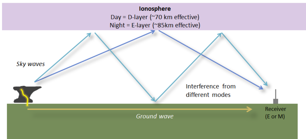
Fig 15.2. Reflection of VLF waves by the ionosphere
