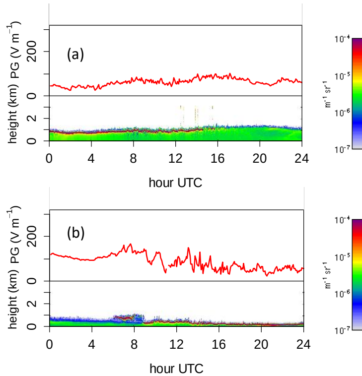
Fig 15.16. Potential Gradient (upper panels, red trace) measured under low stratiform cloud at Reading, observed using a co-located JCI131 field mill and Vaisala CL31 ceilometer (lower panels). (a) Effect of low cloud on the variability in the surface PG on 9 th May 2017, showing the coupling between the cloud base charge and the PG which ceases when the cloud dissipates at about 16UTC. (b) Cloud base charge effect on the surface PG on 15 th March 2016, which leads to a reduction in the PG as the negative charge in the cloud base is brought nearer to the surface with reducing cloud base height. (Ceilometer data are coloured by the backscatter generated according to the colour bar, the cloud base itself yielding the red colour.)
