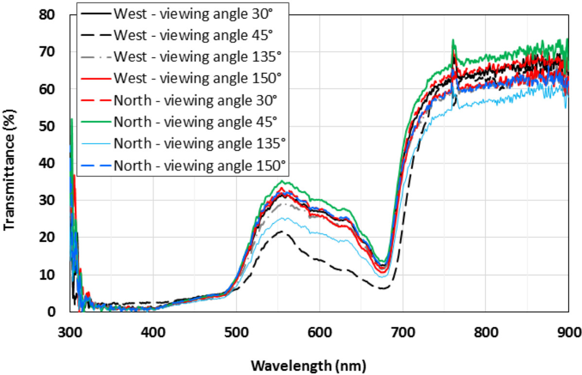
568 Figure 14. Leaf transmission spectra measured from various viewing angles
