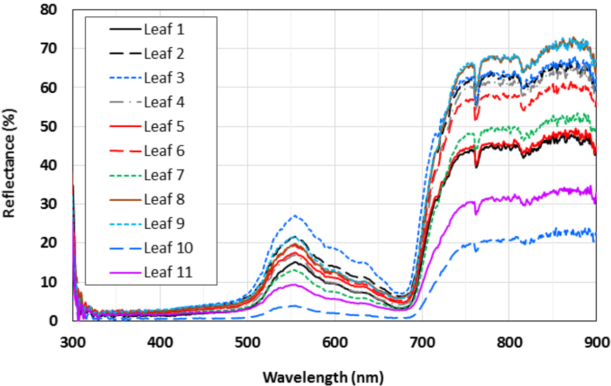
595 596 Figure 16. Leaf-level reflectance measurement on randomly selected leaves which were 597 fully exposed to sunlight
