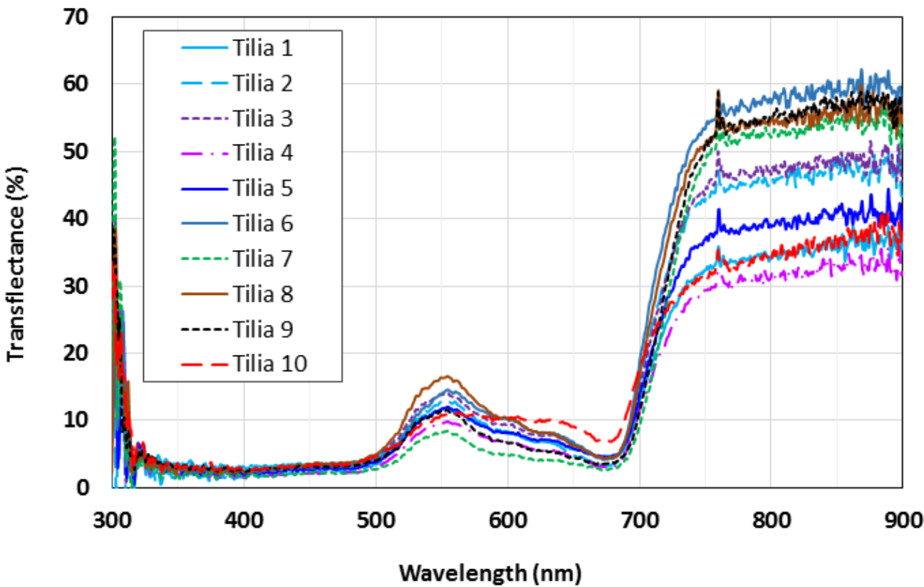
Figure 13. Transflectance spectra of all 10 Tilia trees
