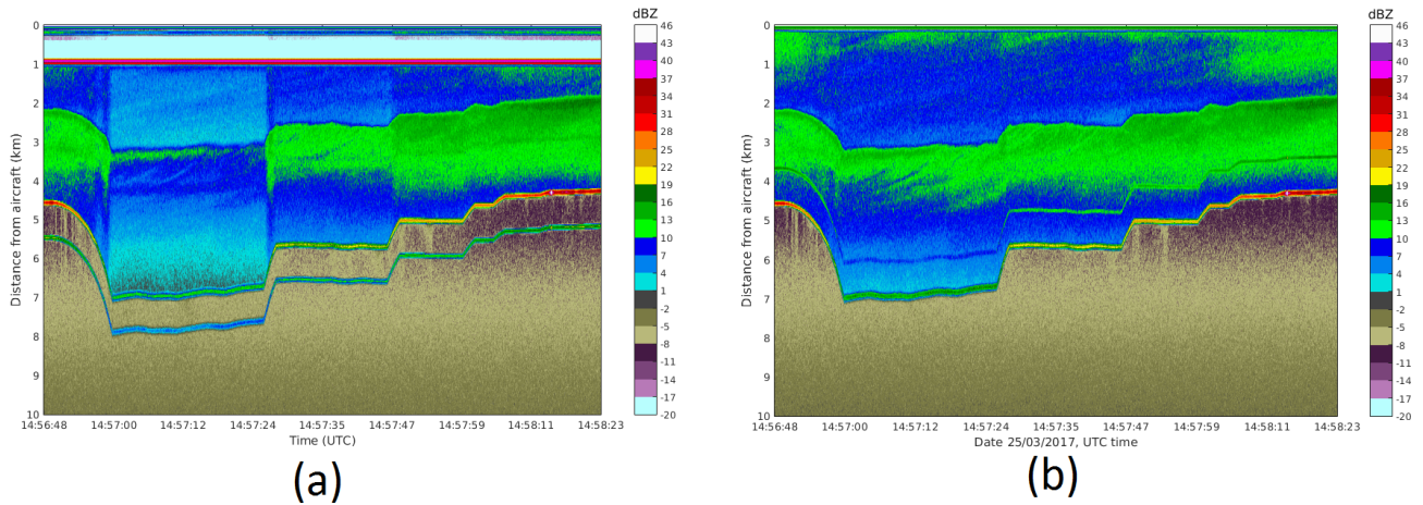
Figure 15. Similar to Fig. 9 but for 25 March flight and in reflectivity space. The PDPP spacing in this case is 6 \mu s.
