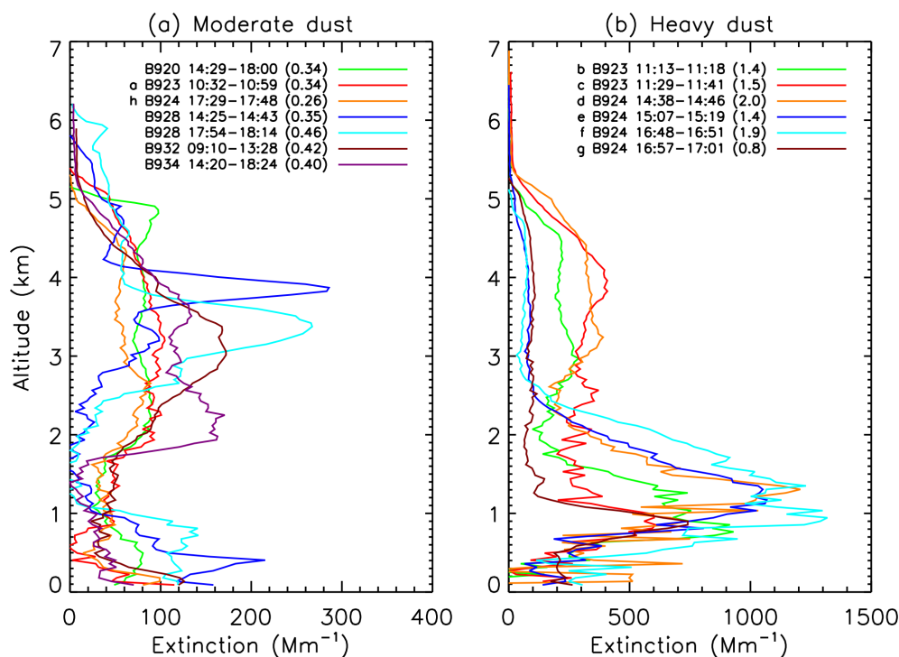
Figure 1. Vertical profiles of the aerosol extinction coefficient measured by airborne lidar, identified by flight number and time (UTC). The number in parentheses is the AOD resulting from the lidar profile. For flights B923 and B924, a letter (a–h) identifies the transects in Fig. 4 used to compute the profiles shown in this figure. Panel (a) refers to the moderate dust conditions, most often encountered during the campaign, whereas panel (b) refers to the heavy dust loads encountered on 12 August.
