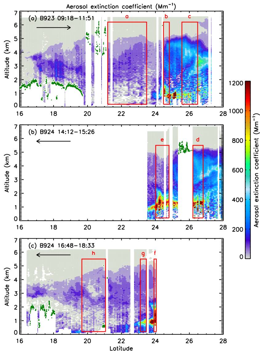
Figure 4. Bi-dimensional structure of the atmosphere on 12 August, for the high-altitude transects: (a) flight B923 from 15 to 28.5° N; (b) first part of B924, from 28.5 to 23.5° N; second part of B924, from 24 to 15° N. This curtain plot is coloured according to the aerosol extinction coefficient measured by lidar at 1 min integration time ( \sim 9 km footprint). The green dots indicate cloud tops detected with the lidar at 2 s integration time ( \sim 300 m horizontal resolution). The red boxes and letters identify the transect portions that have been used to derive the profiles displayed in Fig. 1. The arrows indicate the direction of travel of the aircraft.
