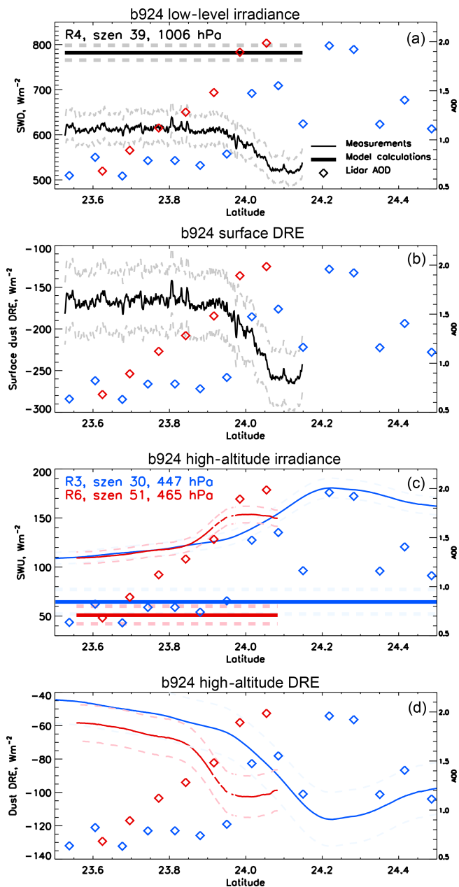
Figure 5. Solar irradiance and instantaneous direct radiative effect of dust ahead of and within the dust front during flight B924. Observations are the thin lines, model clear sky calculations are the bold lines, uncertainties are displayed through dashed lines and lidar AODs are indicated with diamonds. (a) Low-level (run 4, 30 m) measured and modelled shortwave downwelling irradiance; (b) surface direct radiative effect on the shortwave downwelling irradiance; (c) high-altitude shortwave upwelling irradiance for two aircraft legs (run 3, blue; and run 6, red); (d) high-altitude (TOA) direct radiative effect on the shortwave upwelling irradiance for runs 3 and 6.
