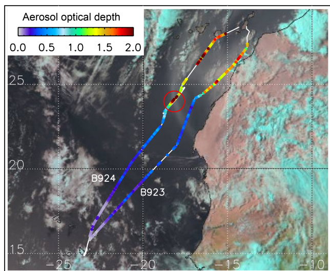
Figure 3. Meteosat Second Generation “321 RGB” image for 12 August at 16:30 UTC, showing the extent of the dust plume advected off the west coast of Africa. The track of flights B923 and B924 is overplotted. A colour scale depicts the lidar-derived AOD, and a red circle indicates the location where the aircraft descended to sample the heavy dust in situ. A SLR at 30 m altitude was performed between 15:52 and 16:04 UTC (run 4), and a SLR at 1000 m took place between 16:09 and 16:29 UTC (run 5).
