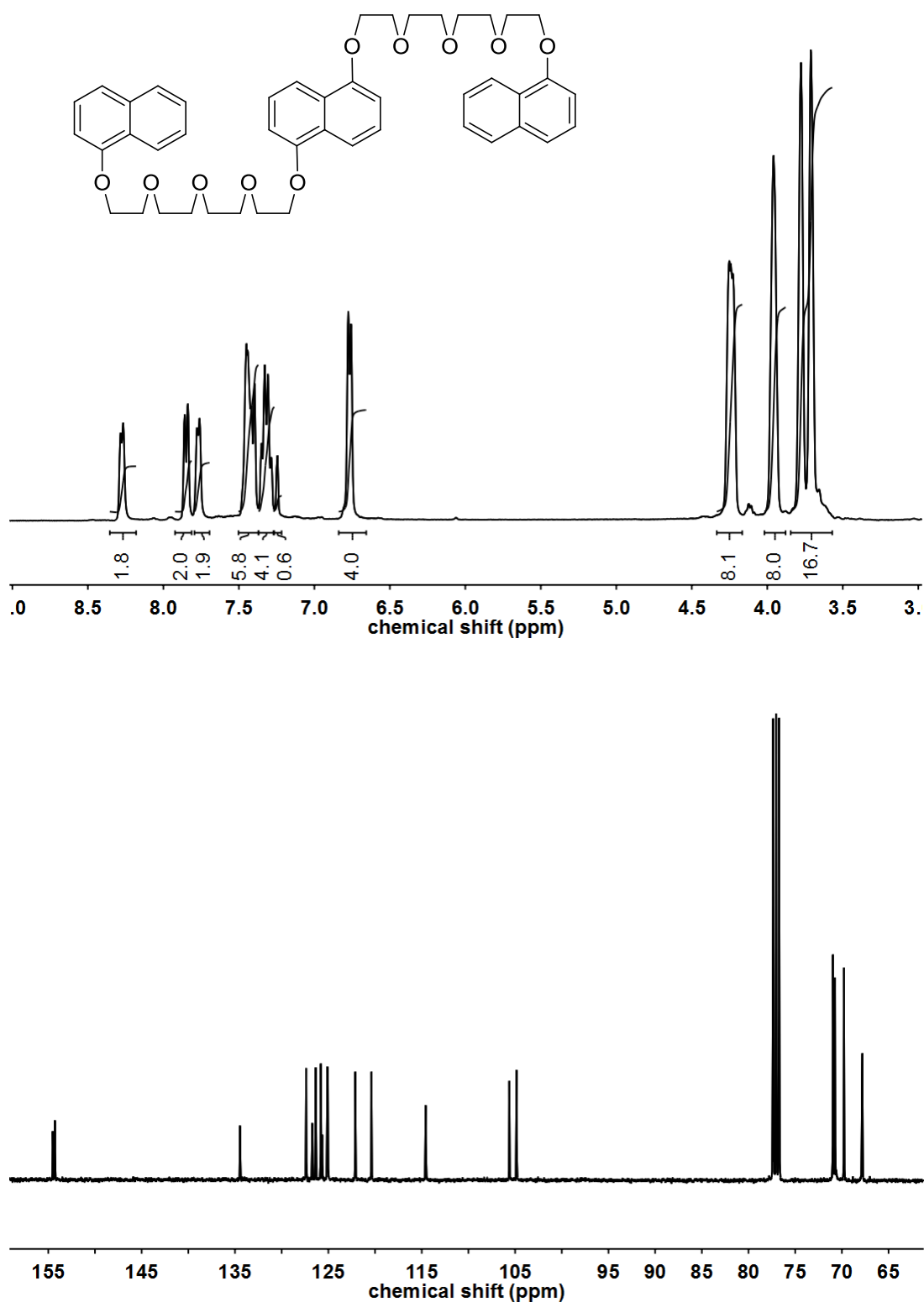
Figure S9. 400 MHz ^1\text{H} and 100 MHz ^{13}\text{C} NMR spectra of 10 ( \text{CDCl}_3 )
