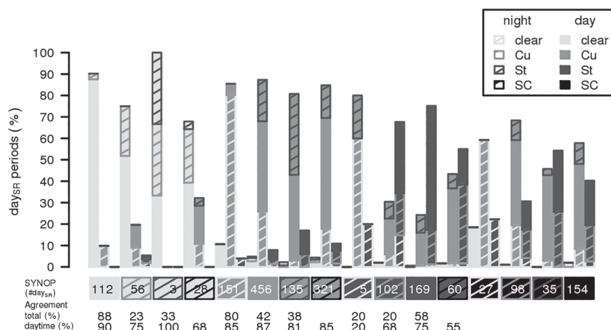
FIGURE 8 Number of 24 hr periods ( \text{days}_R ) centred at sunrise classified into major ABL-classes: Clear, Cu, and St, based on ALC observations for day (fill colour) and night (striped shading). ALC classes are grouped based on SYNOPSIS categories (which also include a stratocumulus (SC) class). Number of periods in ALC class are normalised by total occurrence of the respective SYNOPSIS class (no. of \text{days}_R periods). Agreement (%) is given for the total \text{days}_R period and daytime only
