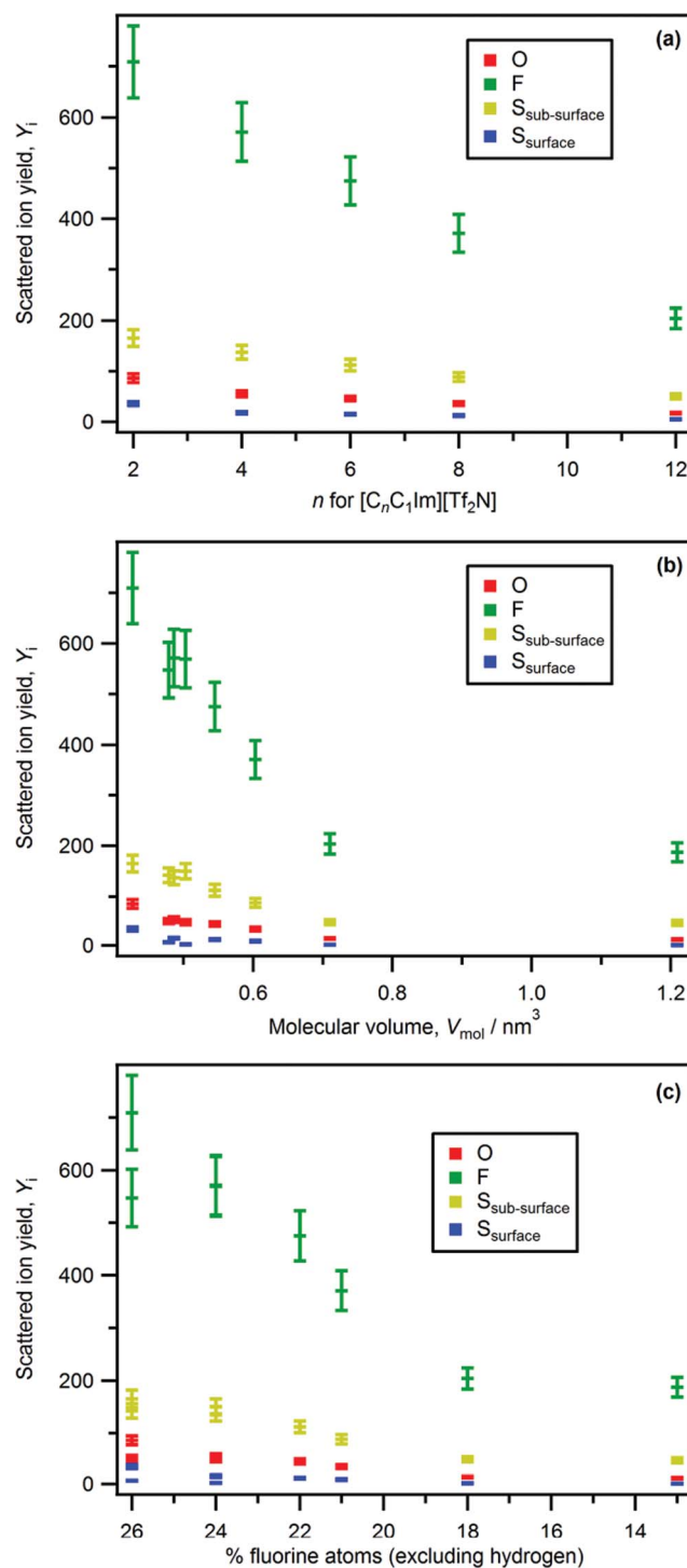
Fig. 8 Scattered ion yield, Y_i , for [C_nC_1Im][Tf_2N] , [C_4C_1Pyr][Tf_2N] , [N_{4,1,1,1}][Tf_2N] and [P_{6,6,6,14}][Tf_2N] vs.: (a) n for [C_nC_1Im][Tf_2N] , (b) molecular volume, V_{mol} , (c) percentage of fluorine atoms (excluding hydrogen atoms).
