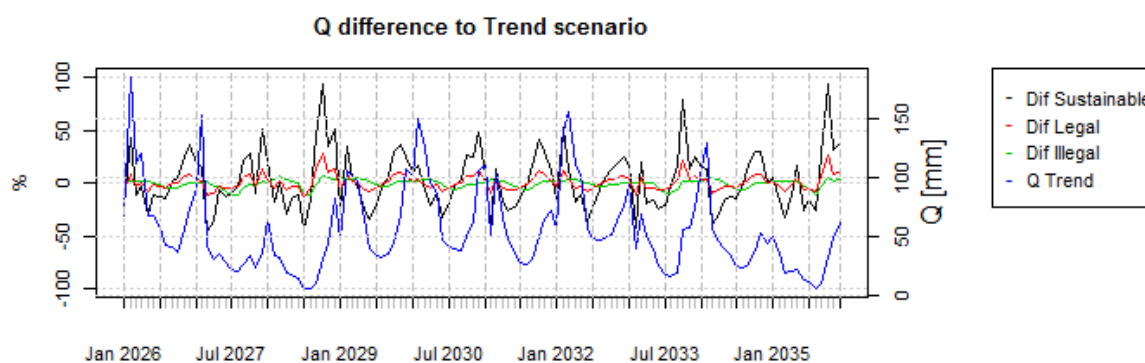
Figure 4 a: Difference in scenario predicted stream discharge: \Delta Q = Q_{trend} - Q_{other\ scenarios} , and simulated stream discharge for trend scenario, das Mortes catchment
