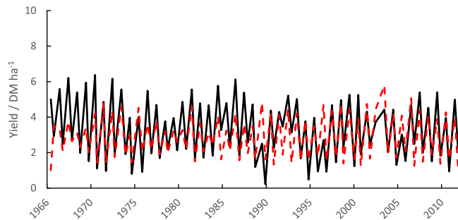
Fig. 9. Simulated (red dashes) and measured (black lines) yields for plots 3a and 14/2a Park Grass permanent grassland experiment, showing both cuts each year.
