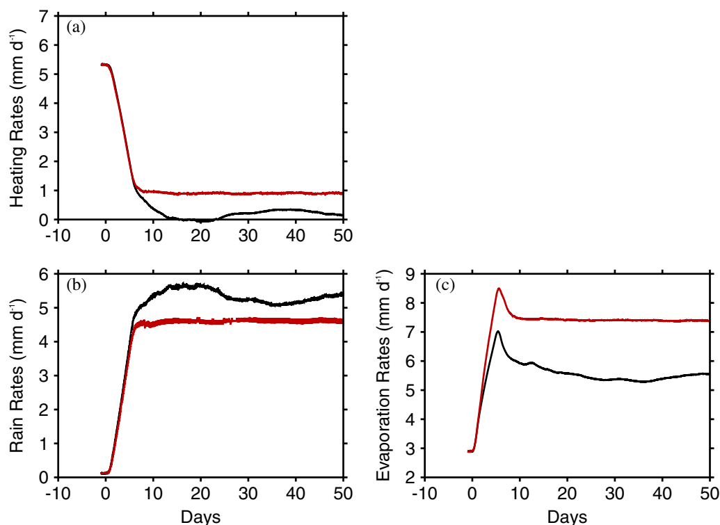
Figure 9. Time evolution of (a) column-integrated heating rates from the large-scale circulation, (b) rain rates, and (c) surface evaporation. Results are the 5 day running mean and five member ensemble mean for the dry column of experiments 1 (black curves) and 1b (red curves). The heating rate is expressed in millimeters per day via the latent heat of vaporization in order to allow easy comparison.
