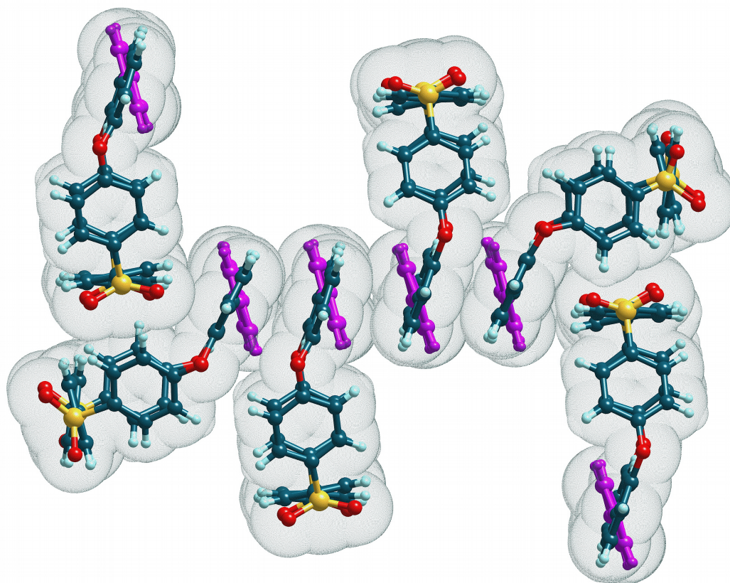
Figure 4. Termination of the quadruple \pi -stack motif in the crystal of the macrocyclic radical-cation 1b , showing van der Waals surfaces. Viologen units are highlighted in magenta. Each "terminating" macrocycle is itself a component of a further quadruple \pi -stack.
