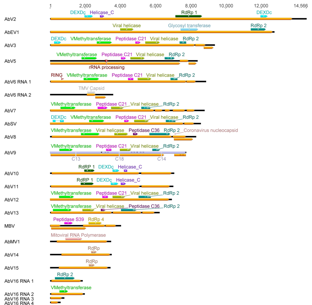
Figure 1. The genome organisation and protein coding potential of the viruses. ORFs greater than 300 bases on the + strand are shown as yellow annotations. Grey annotations indicate assembled contigs. Protein domains identified by NCBI Conserved Domain Search (E-value threshold 0.01) or HHPRED ( p < 10^{-3} ) are shown as annotations in other colours. Incomplete annotations are shown with a jagged edge. Scale is length in bases.
