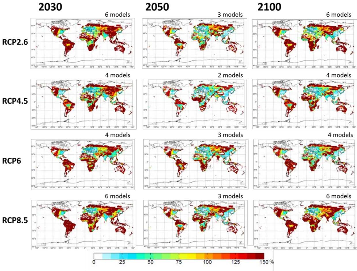
Figure S9 – Spatial distribution of model variability in future premature mortality (IHD+STROKE+COPD+LC) for PM 2.5 calculated as a sum of species for all RCP scenarios in 2030, 2050 and 2100, showing the coefficient of variation of mortality estimates in each grid cell.
