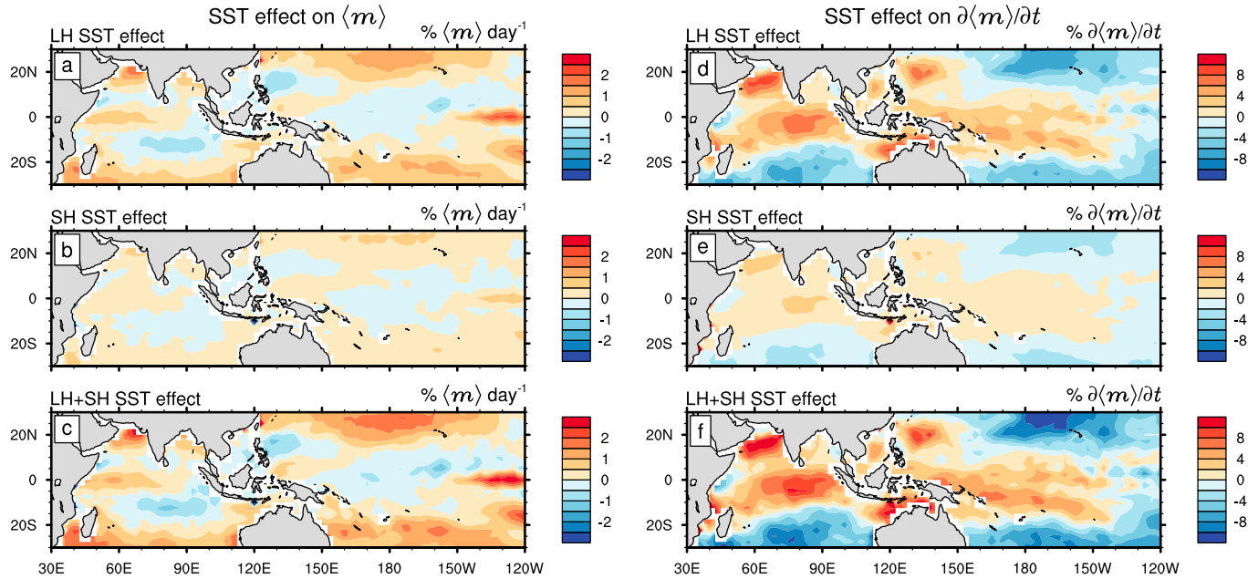
Figure 12. The SST effect on \langle m \rangle (left column) and \partial \langle m \rangle / \partial t (right column) for (a, d) LH*, (b, e) SH*, and (c, f) their sum. As in Figure 11i, the SST effect is calculated as the difference between F_m(\text{LH}_{\text{SST}}^* + \text{SH}_{\text{SST}}^*) and F_m(\text{LH}_{\text{SST}}^* + \text{SH}_{\text{SST}}^*) , and F_{\partial m / \partial t}(\text{LH}_{\text{SST}}^* + \text{SH}_{\text{SST}}^*) and F_{\partial m / \partial t}(\text{LH}_{\text{SST}}^* + \text{SH}_{\text{SST}}^*) , respectively.
