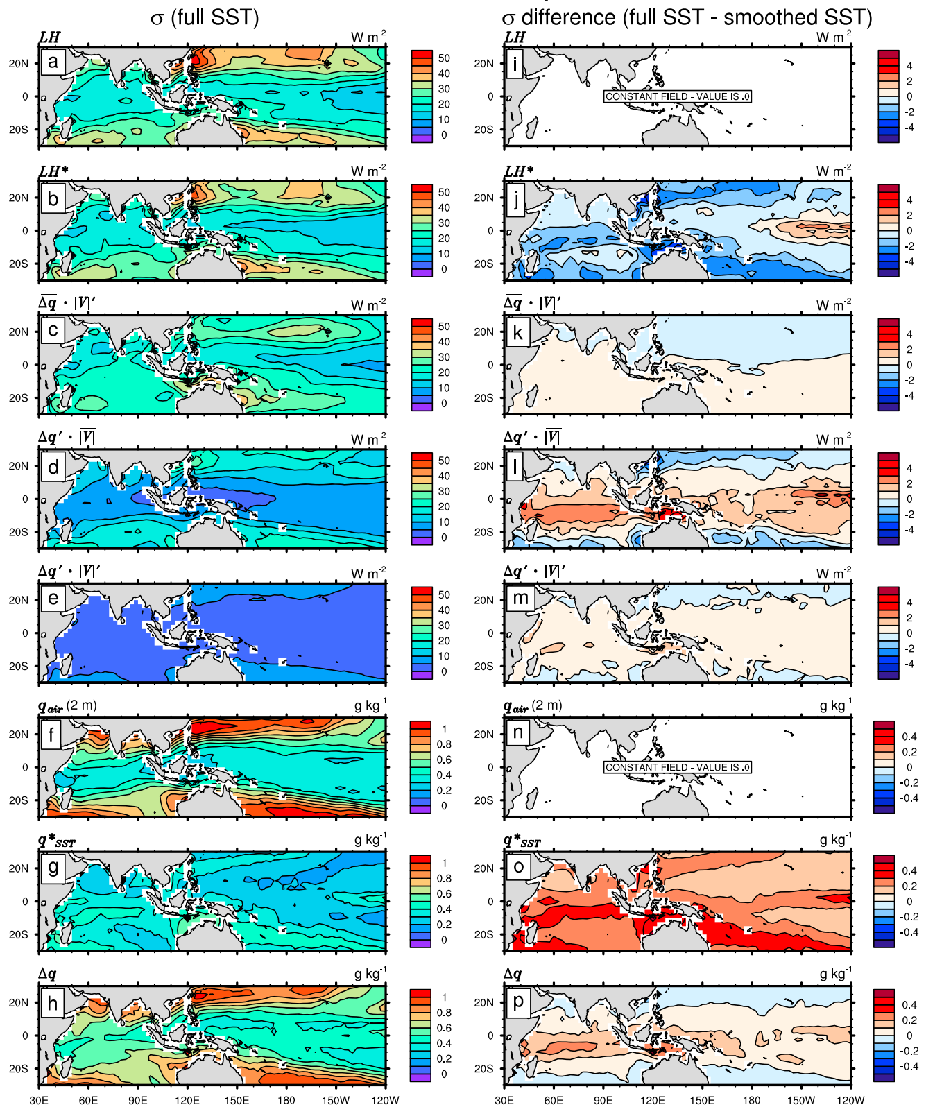
Figure 5. November–April 20–100 day filtered standard deviation of (a) LH; (b) LH*; (c) \overline{\Delta q} \cdot |\mathbf{V}|' ; (d) \Delta q' \cdot |\mathbf{V}| ; (e) \Delta q' \cdot |\mathbf{V}|' ; (f) q_{\text{air}} ; (g) q_{\text{ssr}}^* ; and (h) \Delta q . In Figures 5b–5h quantities are computed using the “full” SST time series. In Figures 5i–5o the difference between values are plotted in the left column and those computed using 61 day running-mean SST.
