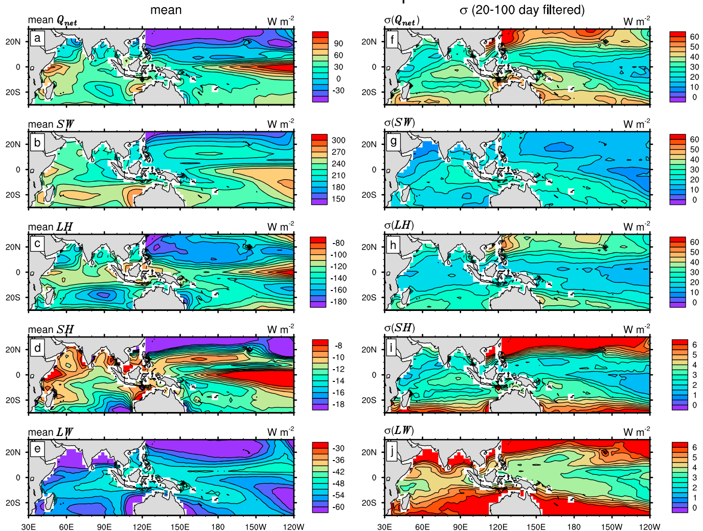
Figure 4. As in Figure 3, but for (a, f) Q_{net} , (b, g) net surface shortwave radiation, (c, h) LH, (d, i) SH, and (e, j) net surface longwave radiation. The 850 hPa zonal winds are omitted. In Figures 4a–4e, positive fluxes warm the ocean.
