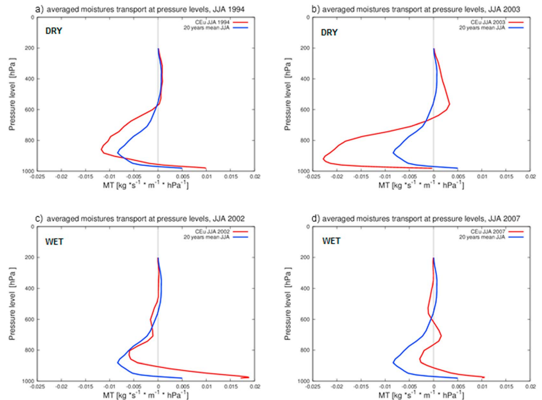
Figure 7. Vertical structure of horizontal moisture transport over CE region during selected anomalously (a, b) dry and (c, d) wet summers (red) and the JJA mean profile (blue). Positive (negative) values indicate resulting moisture transport into (out of) the region.
