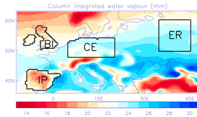
Figure 1. Summer (JJA) mean CWV distribution over Europe. Black curves indicate boundaries of the regions under analysis.
