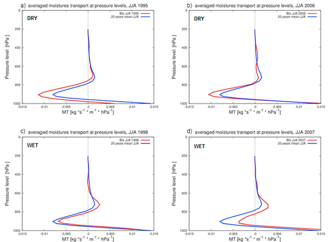
Figure 6. Vertical structure of horizontal moisture transport over BI region during selected anomalously (a, b) dry and (c, d) wet summers (red) and the JJA mean profile (blue). Positive (negative) values indicate resulting moisture transport into (out of) the region.
