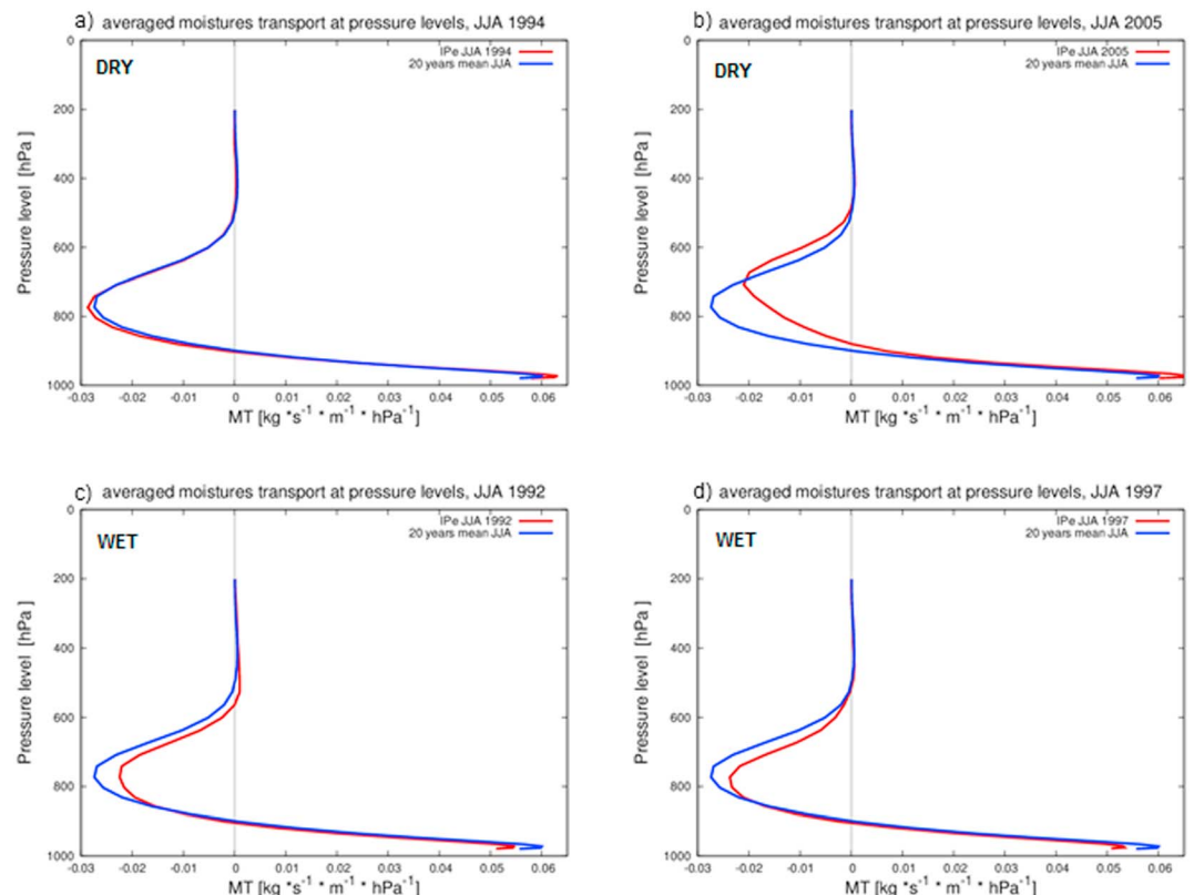
Figure 5. Vertical structure of horizontal moisture transport over IP region during selected anomalously (a, b) dry and (c, d) wet summers (red) and the JJA mean profile (blue). Positive (negative) values indicate resulting moisture flux into (out of) the region.
