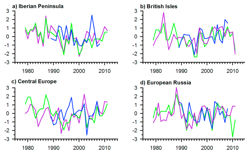
Figure 3. Regional time series of normalized anomalies of seasonal mean summer CWV (violet curve), CWV_{rat} (green curve), and horizontal moisture transport (blue curve).
