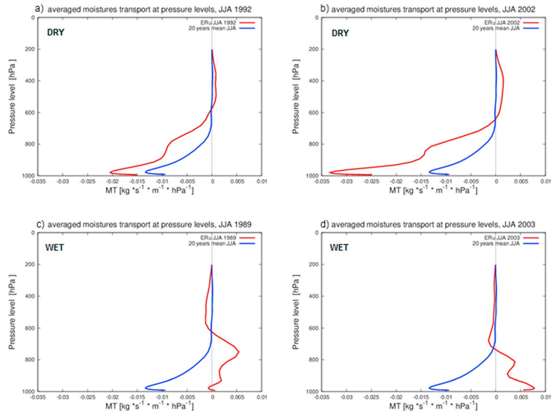
Figure 8. Vertical structure of horizontal moisture transport over ER region during selected anomalously (a, b) dry and (c, d) wet summers (red) and the JJA mean profile (blue). Positive (negative) values indicate resulting moisture transport into (out of) the region.
