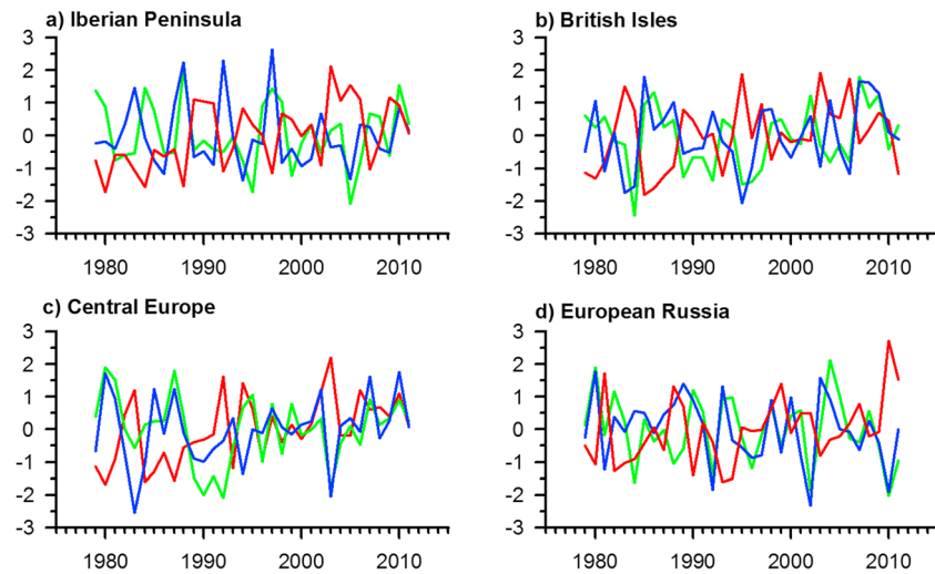
Figure 2. Regional time series of normalized anomalies of seasonal mean summer precipitation (blue curve), soil moisture (green curve), and air temperature (red curve).
