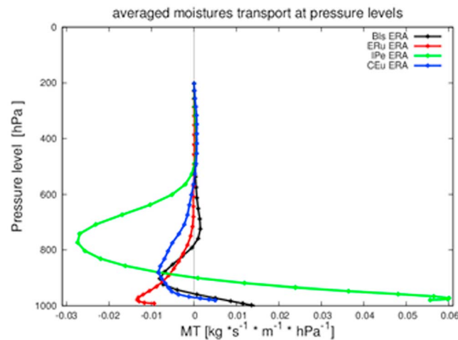
Figure 4. Climatological vertical structure of summertime (JJA) horizontal moisture transport over four European regions. Positive (negative) values indicate resulting net moisture transport into (out of) the region at particular level.
