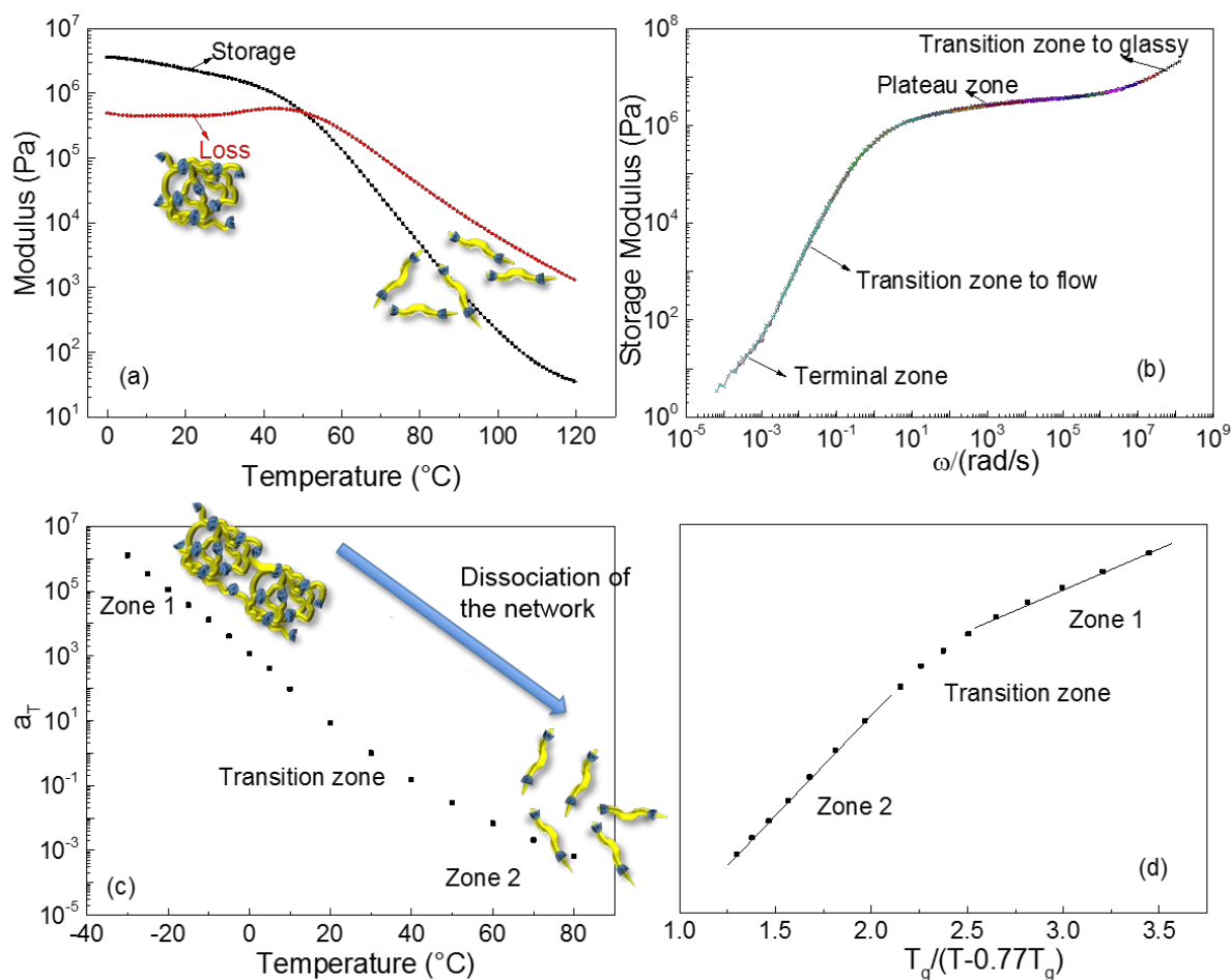
Fig. 2 The rheological behaviour of polyurethane 1 . a) temperature sweep at 5 Hz; b) master curve at a reference temperature of 30 ^{\circ}\text{C} , different colours corresponding to different temperatures; c) time-temperature shift factor a_T of polyurethane 1 as a function of temperature; d) plot of a_T for polyurethane 1 as a function of temperature normalized to T_g .
