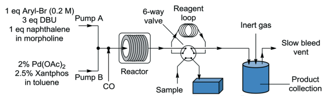
Fig. 1 System diagram.
