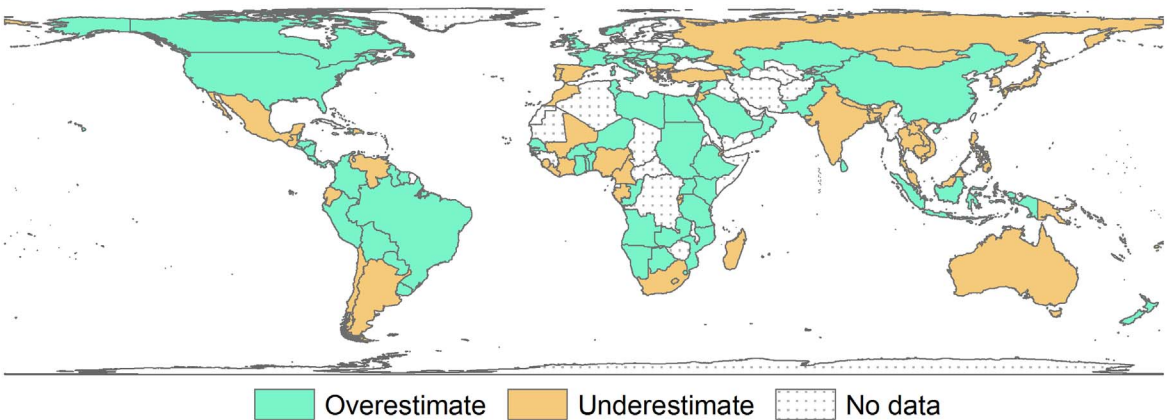
Fig. 2. Observed (a) and predicted (b) number of threatened mammal species per country. Panel (c) represents the differences between predicted and observed values divided by the total mammalian richness of the country. Both overestimated and underestimated values are within the \pm 0.14\% range; except for Cyprus, Indonesia, Barbados, Seychelles, New Zealand and Mauritius that present overestimates > 0.14\% . No data indicates that selected socioeconomic indicators were not available for those countries.
