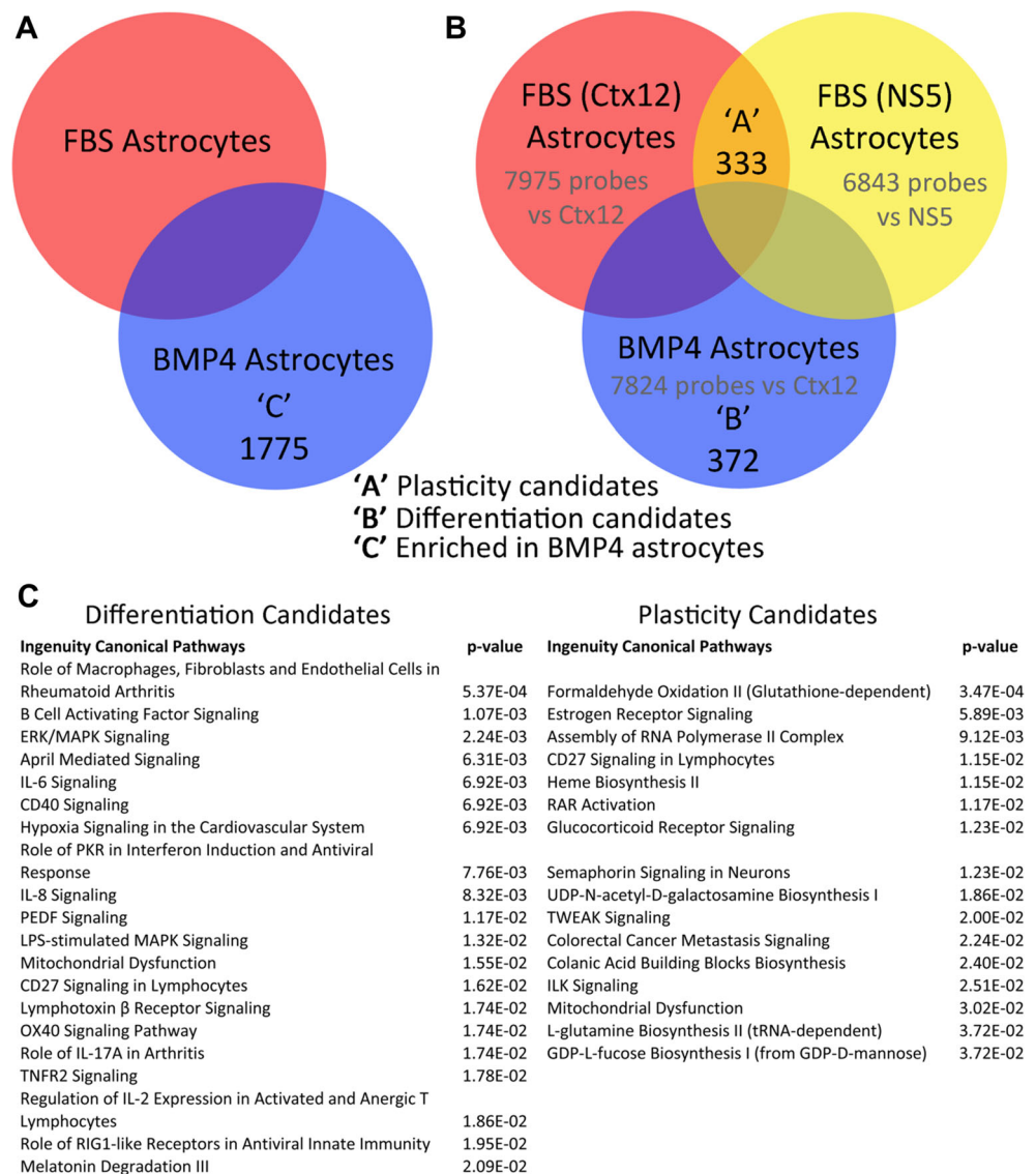
Fig. 2 Candidate genes and signalling pathways involved in phenotype and potential of specific astrocyte populations. a Venn diagram showing number of genes expressed at a significantly different level between BMP4 and FBS astrocytes. b Venn diagram showing genes whose expressions were significantly changed in FBS- or BMP4-derived astrocytes compared to undifferentiated CTX12 or NS5 cells (FDR<0.05). c Top canonical pathways enriched in the differentiation candidate gene set 'B' and 'plasticity' candidate gene set 'A' both shown in b
