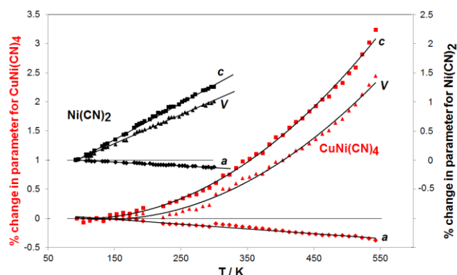
Fig. 6 The relative percentage changes in the a and c lattice parameters and volume, V , for \text{CuNi(CN)}_4 and \text{Ni(CN)}_2 over the temperature ranges (93 – 543) K and (95 – 295) K, respectively. The relative % change of a parameter, l_{T2} , is given by 100 \times (l_{T2} - l_{T1})/l_{T1} , where l_{T2} is the parameter l at temperature T_2 , and l_{T1} is the parameter l at the lowest temperature, T_1 .
