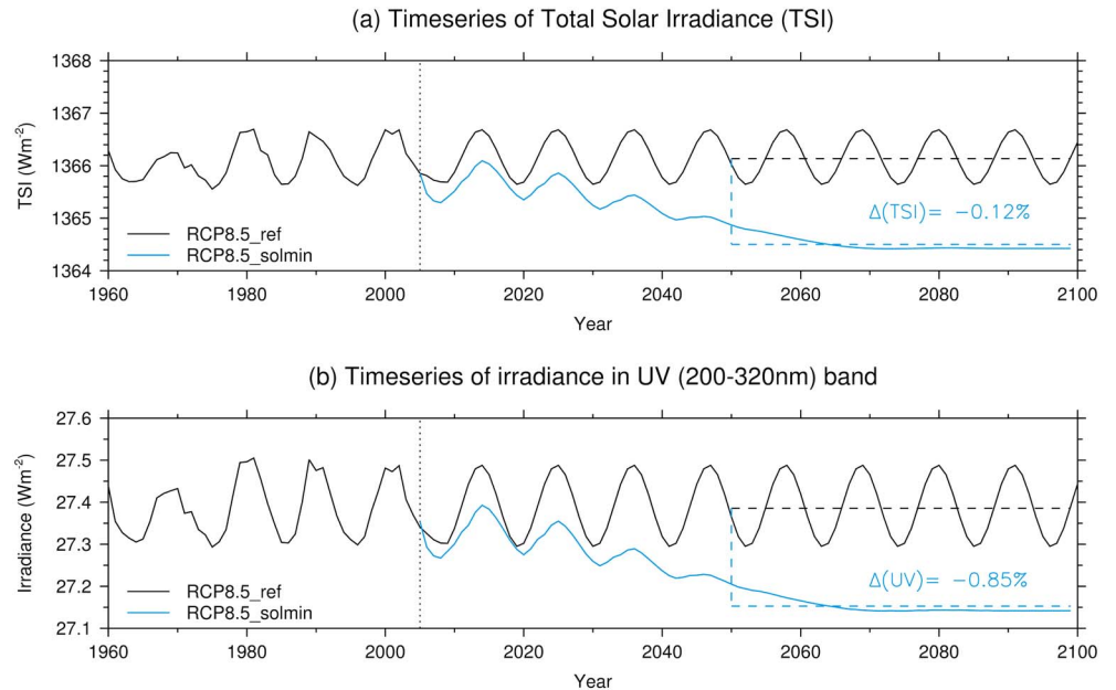
Figure 1. Time series of (a) TSI ( \text{W m}^{-2} ) and (b) the irradiance in the 200–320 nm spectral band ( \text{W m}^{-2} ) for the RCP8.5_ref (black) and RCP8.5_solmin (blue) cases. The mean percent differences for the period 2050–2099 are shown in the legends.
