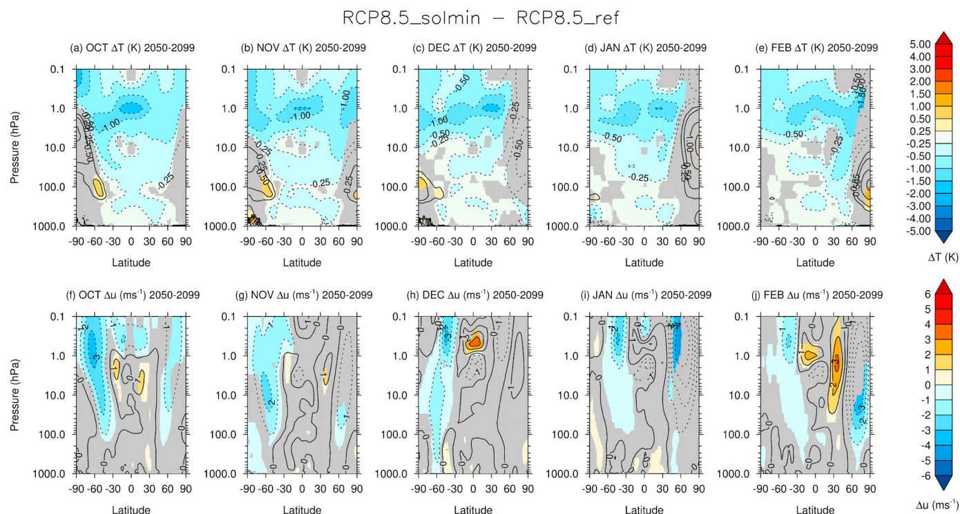
Figure 5. The difference in monthly mean (a–e) \bar{T} (K) and (f–j) \bar{u} ( \text{m s}^{-1} ) for the period 2050–2099 between the RCP8.5_solmin and RCP8.5_ref experiments. The panels show data for October–February, respectively. The grey shading denotes regions where the differences are not statistically significant at the 95% confidence level.
