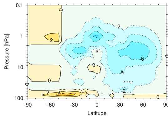
Figure 2. The percent differences in ozone between the RCP8.5_solmin and the RCP8.5_ref experiments for the period 2050–2099. The changes are based on the CMIP5-recommended ozone database described by Cionni et al. [2011] [see also Schmidt et al. , 2013]. No changes are imposed at pressures higher than \sim 100 hPa.
