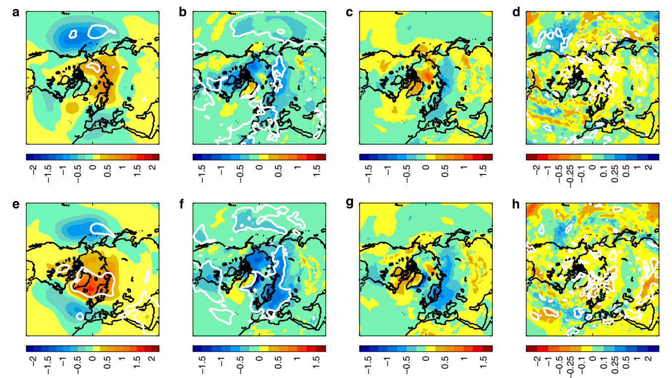
Figure 3 | Winter climate response for future solar minimum experiments. Differences between experiments and CTRL-8.5 for the period 2050–2099 for (a,e) sea-level pressure (hPa), (b,f) near-surface temperature (°C), (d,h) precipitation (mm day -1 ). (c,g) They are as in b and f but with control lagged by 2 years to give similar global mean temperature. Upper panel plots are for EXPT-A and lower panel plots are for EXPT-B. Anomalies are for December to February. Solid white contours indicate significance with a 95% confidence interval.
