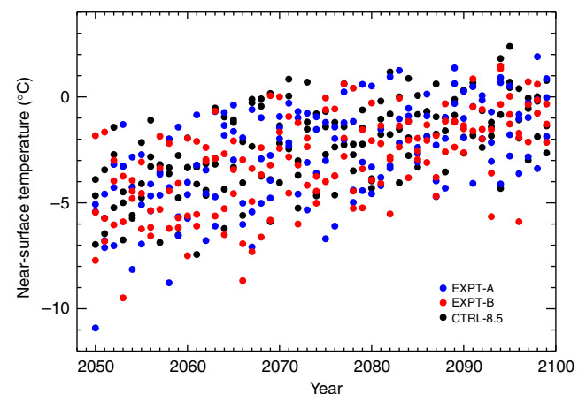
Figure 7 | Variability in modelled European winter temperatures. Winter (December to January) northern European ( 10^{\circ}\text{W} – 40^{\circ}\text{E} , 48 – 75^{\circ}\text{N} ) near-surface temperatures ( ^{\circ}\text{C} , land points only) for 2050 to 2099 for individual ensemble members of EXPT-A (blue), EXPT-B (red) and CTRL-8.5 (black).
