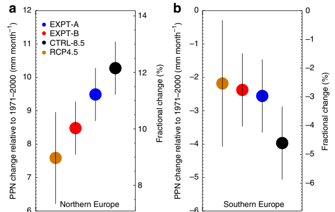
Figure 6 | Winter European precipitation response. Mean winter (December to February) European precipitation change ( \text{mm month}^{-1} ) for 2050–2099 for future scenarios relative to the historical simulation (1971–2000) for (a) northern Europe ( 10^{\circ}\text{W} – 30^{\circ}\text{E} , 45 – 65^{\circ}\text{N} ) and (b) southern Europe ( 10^{\circ}\text{W} – 30^{\circ}\text{E} , 35 – 45^{\circ}\text{N} ). Whiskers show the s.e. Differences between EXPT-B and CTRL-8.5 are significant with a 90% (75%) confidence interval for northern Europe (southern Europe).
