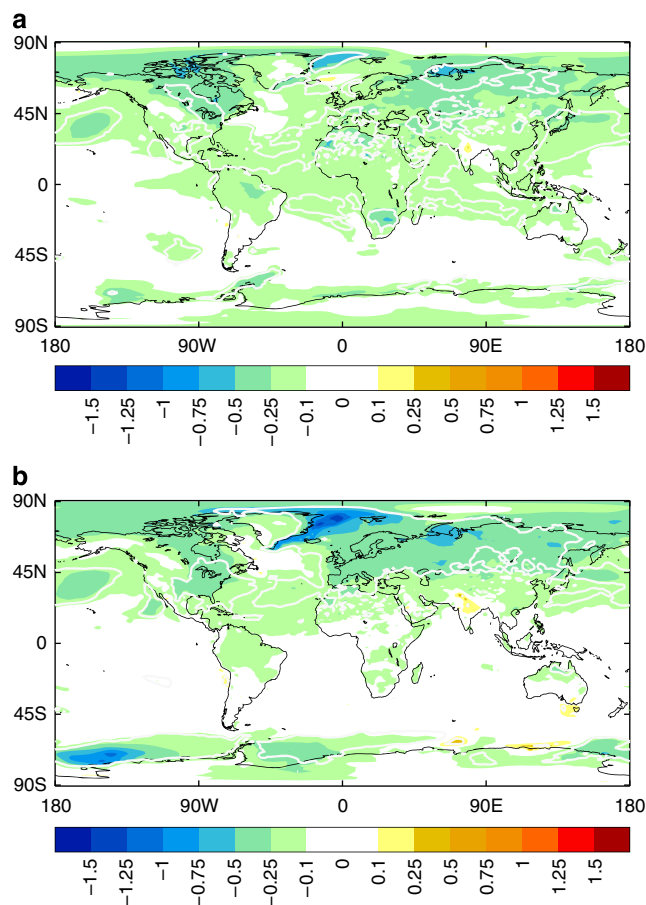
Figure 2 | Annual mean surface temperature response for future solar experiments. Difference in near-surface temperature (°C) between (a) EXPT-A and (b) EXPT-B and CTRL-8.5 for the period 2050–2099. Solid white contours indicate significance with a 95% confidence interval.
