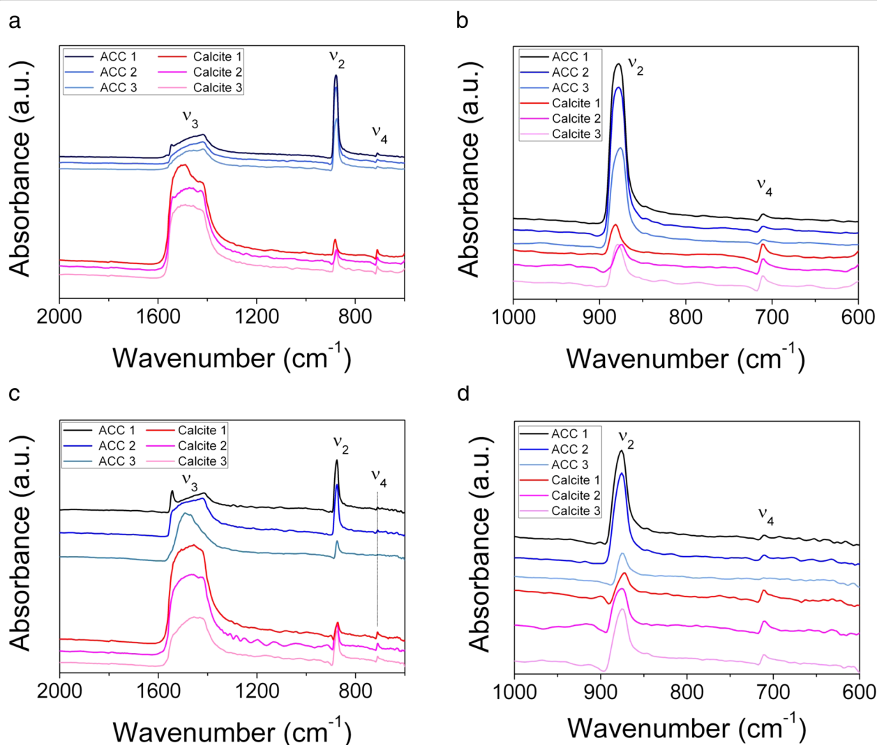
Figure 7 Typical \mu -FTIR spectra obtained from granules. a, b) Typical \mu -FTIR spectra obtained from ACC-rich and calcite-rich regions of granule Fresh-1 imaged in Figure 5; c, d) Typical \mu -FTIR spectra obtained from ACC-rich and calcite-rich regions of granule Old-2 imaged in Figure 6. Samples are offset on the vertical axis for clarity.
