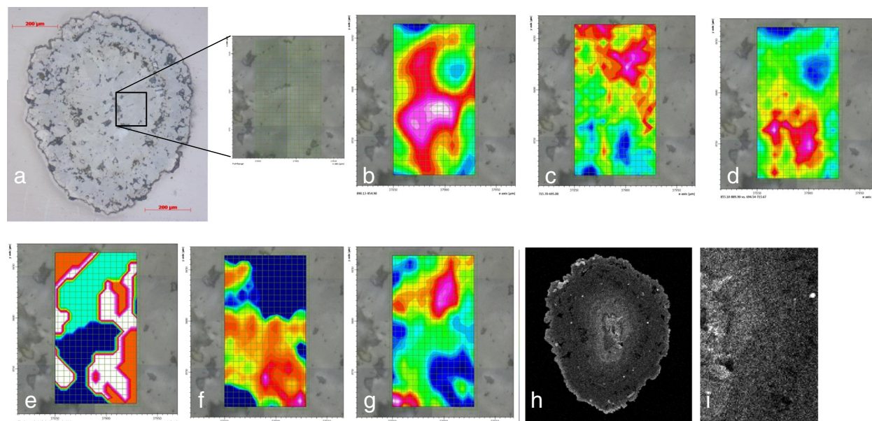
Figure 6 Images and intensity maps from analysis of a thin section of granule Old-2. a) reflected light image of an area of granule Old-2 resident in soil for between 1 and 39 days, scale bar is 100 µm; high spatial-resolution µ-FTIR intensity maps for (b) \nu_2 (855–890 \text{cm}^{-1} ), (c) \nu_4 (695–716 \text{cm}^{-1} ) and (d) \nu_2/\nu_4 ratio map with high intensity areas indicative of ACC rich regions, e) cluster analysis map showing 4 clusters (dark blue, light blue, orange and white), f) component regression intensity map for ACC, g) component regression intensity map for calcite, h) electron microprobe Mn distribution map, i) close up of (h) focussing on area of µ-FTIR maps showing lack of correlation between elemental and ACC variation. For µ-FTIR intensity maps, red indicates high intensity, blue indicates low intensity while for the elemental maps bright indicates higher concentrations.
