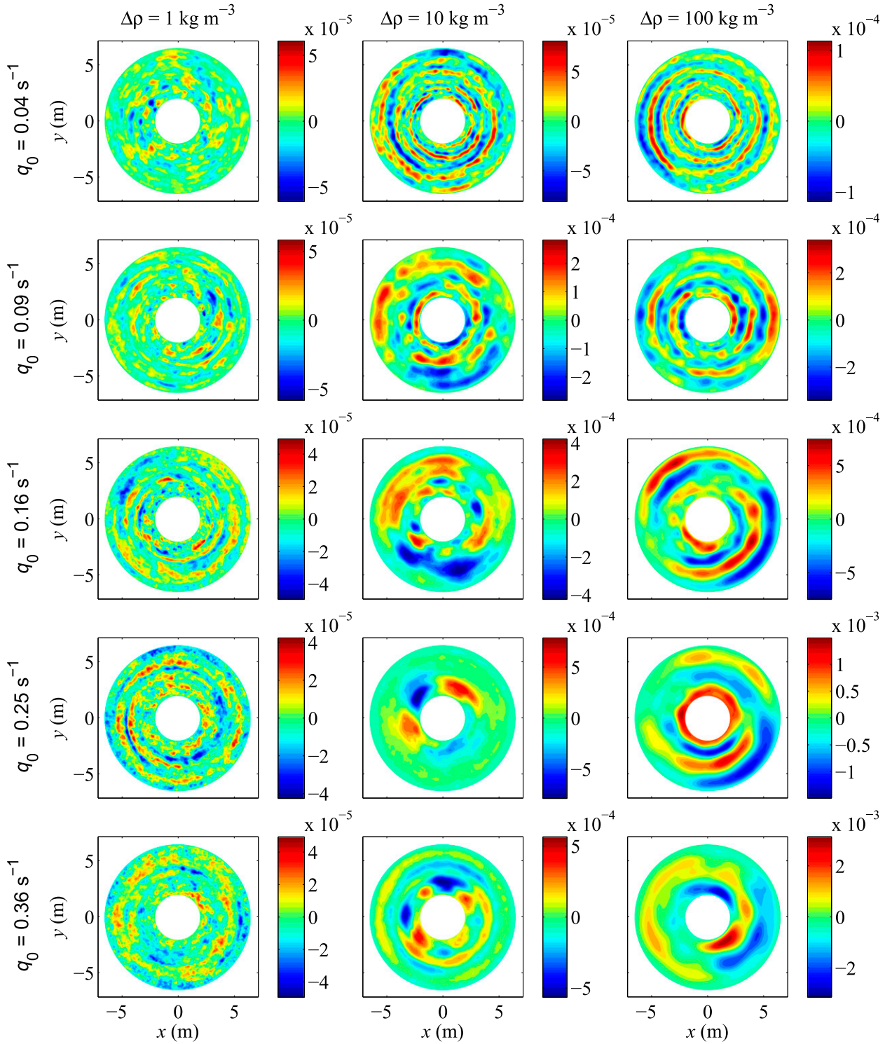
FIG. 9. Baroclinic streamfunction (m 2 s -1 ) after 100 000 s for each combination of \Delta\rho and q_0 , that is, for simulations (left) 1–5, (middle) 6–10, and (right) 11–15.
