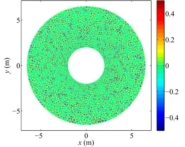
FIG. 2. An example of the initial condition on q_i + fsr/H in either of the layers ( \text{s}^{-1} ). A noise field of amplitude q_0 = 1.0 \text{ s}^{-1} has been bandpass filtered to permit wavelengths mainly between 5 and 10 times the grid spacing, as described in section 2b.
