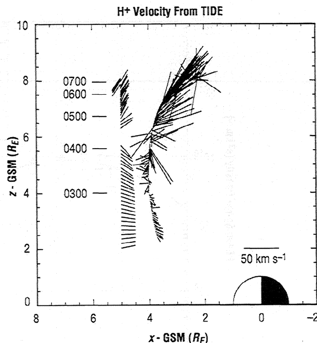
Figure 4. H^+ velocities and the direction of the local magnetic field in the GSM x - z plane for May 29, 1996, 0230–0800 UT (1 min average). The ion velocities (plotted on the right) are referenced to the satellite track. The magnetic field direction is plotted as unit vectors with their tails anchored at x = 5 .
