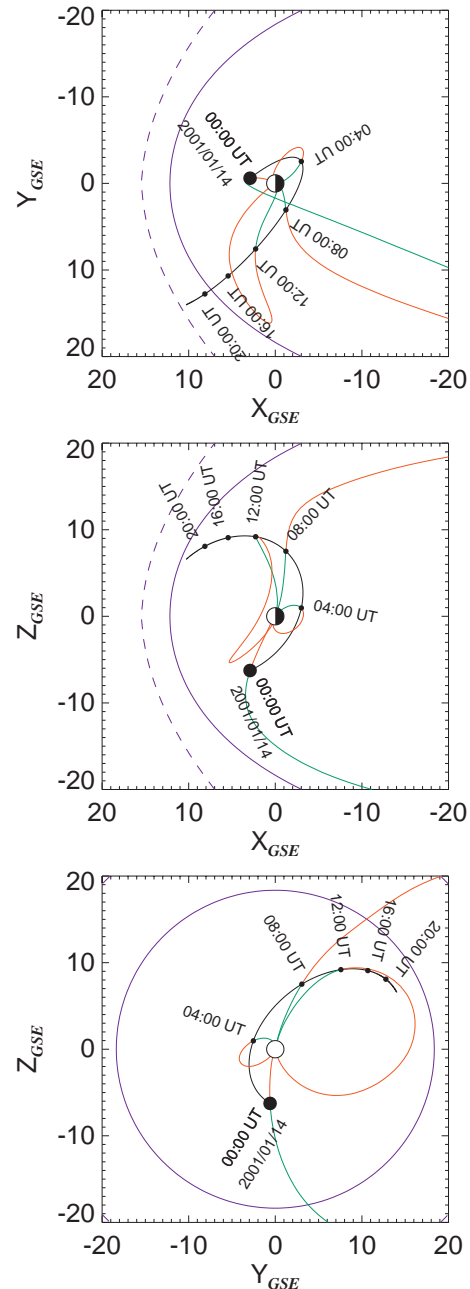
Fig. 2. The Cluster orbit in Geocentric Solar Ecliptic ( X_{\text{GSE}} , Y_{\text{GSE}} , Z_{\text{GSE}} ) coordinates (in black) along with the mapped field lines that give ionospheric footprints, such as that shown in Fig. 1. (a), (b) and (c) are projections onto the ( X_{\text{GSE}} , Y_{\text{GSE}} ), ( X_{\text{GSE}} , Z_{\text{GSE}} ) and ( Y_{\text{GSE}} , Z_{\text{GSE}} ) planes and the solid and dashed blue lines show the model magnetopause and bow shock locations for Z_{\text{GSE}} = 0 , Y_{\text{GSE}} = 0 , and X_{\text{GSE}} = 0 , respectively, predicted using the magnetopause model by Shue et al. (1997) and the bow shock model by Peredo et al. (1995). Traced field lines are shown from the spacecraft locations at 04:00, 08:00 and 12:00 UT. Field lines mapped to the local (northern) hemisphere are shown in green, and those mapped to the southern hemisphere are in red.
