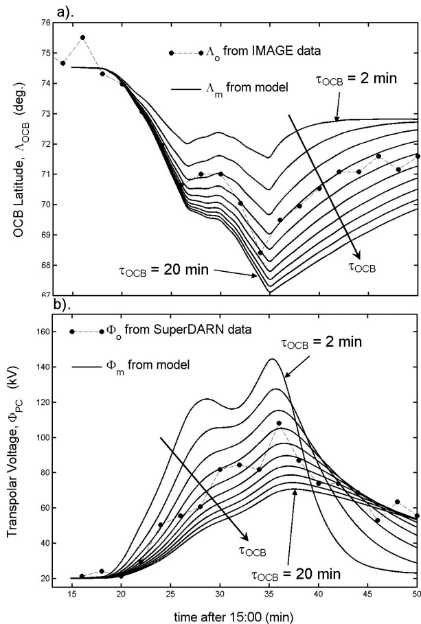
Figure 4. Observed and modeled variations of (a) the latitude of the noon open-closed boundary \Lambda_{\text{OCB}} and (b) the transpolar voltage \Phi_{\text{PC}} . The dashed lines connecting dots are the observed values ( \Lambda_o and \Phi_o ) and the solid lines are modeled variations ( \Lambda_m and \Phi_m ) for various boundary relaxation time constants, \tau_{\text{OCB}} . Curves are for \tau_{\text{OCB}} of 2–20 min, in steps of 2 min. The peak electric field employed is E_{\text{no}} = 114 \text{ mV m}^{-1} .
