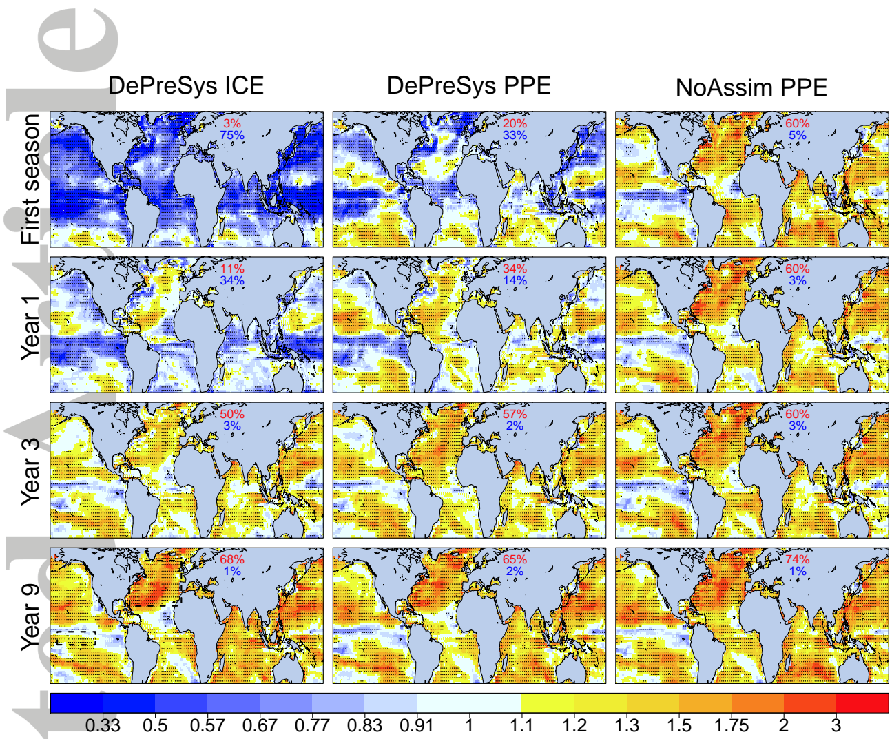
Figure 1. Spread-error ratio (ratio of mean intra-ensemble standard deviation and root mean squared error of ensemble mean forecasts, adjusted for ensemble size) for the three ensemble experiments for four different forecast lead times. Stippled areas indicate where the ratio is significantly different from one at the 10% level. The number in red (blue) on each panel is the proportion of grid boxes with the spread-error ratio significantly greater (smaller) than one. The boxes in the bottom left panel indicate the regions examined in Figures 3 and S2.
