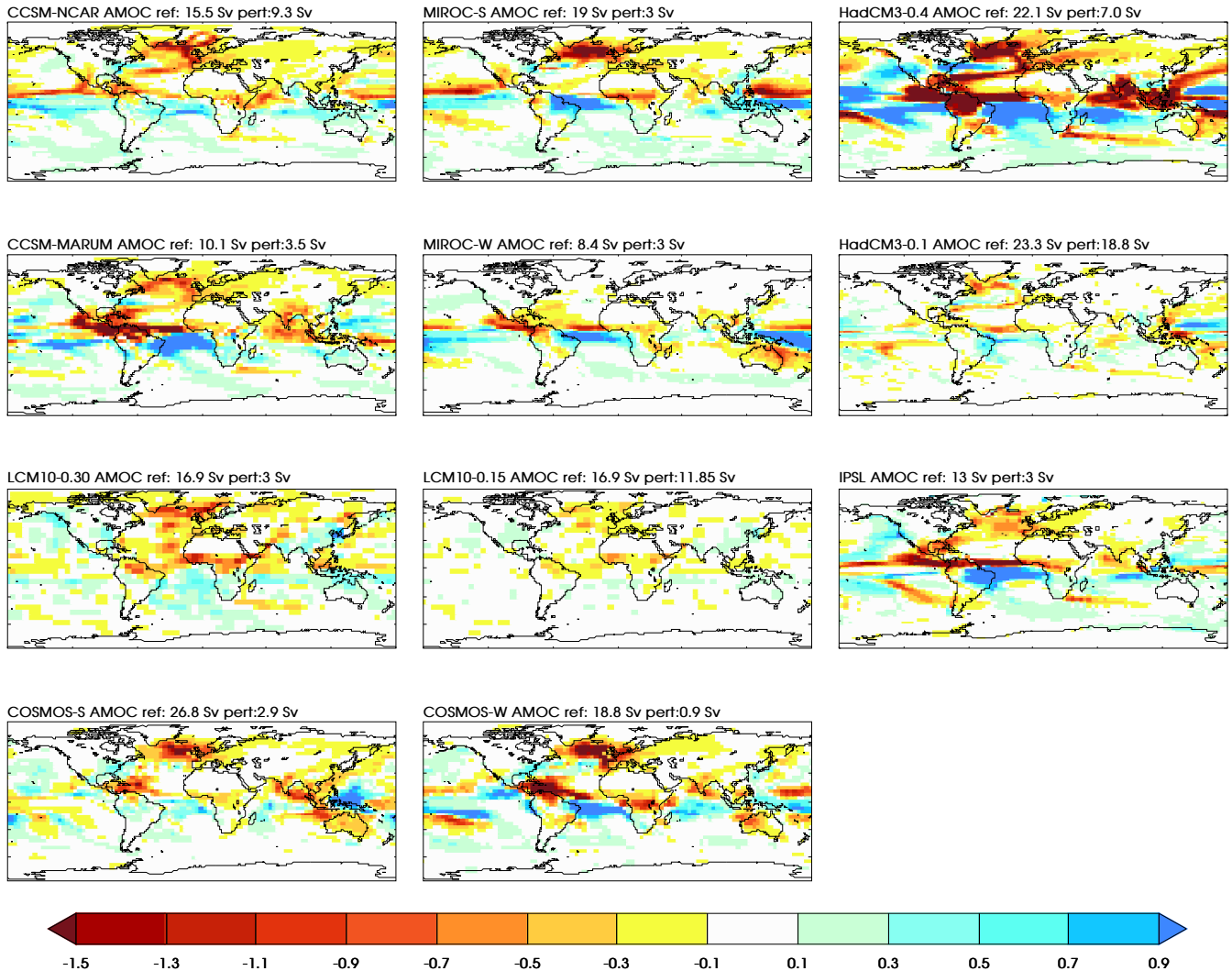
Fig. 4. Same as Fig. 2 for the mean annual precipitation, in mm day -1 .
