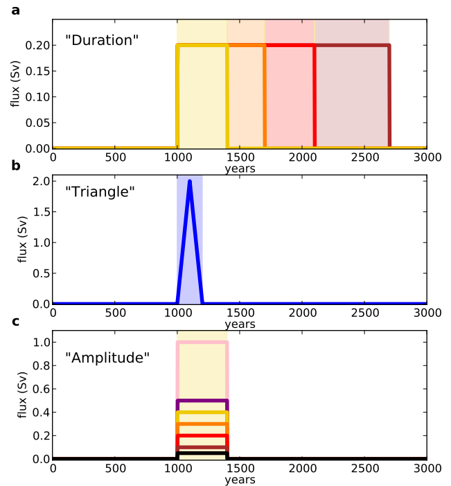
Fig. 1. Evolution of the fresh water flux (Sv) in the three types of experiments: (a) for the “Duration” experiments with fresh water fluxes of 0.2 Sv added during 400, 700, 1100 or 1700 yr, (b) for the “Triangle” experiments with a fresh water flux linearly increasing for 100 yr to 2 Sv, then decreasing again from 100 yr, and (c) for the “Amplitude” experiments with fresh water flux added during 400 yr of 0.05, 0.1, 0.2, 0.3, 0.4, 0.5 or 1 Sv.
