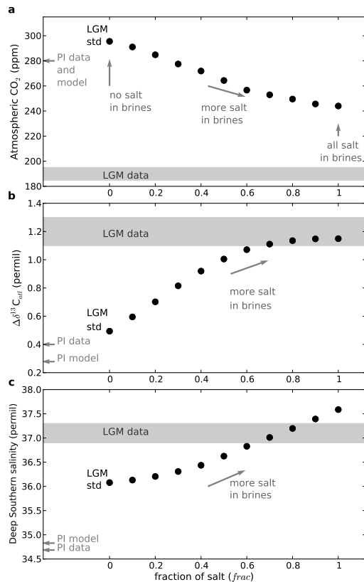
Fig. 2. (a) Atmospheric \text{CO}_2 concentration, (b) \Delta\delta^{13}\text{C}_{\text{atl}} (mean upper ( -2000\text{ m} to 0\text{ m} ) to deep ( -5000\text{ m} to -3000\text{ m} ) gradient in the Atlantic) and (c) salinity in the deep Southern ocean (Atlantic sector, 50^\circ\text{S} , 3626\text{ m} depth) as a function of the fraction of salt released by sea ice formation used for the brine mechanism (fraction of salt \text{frac} , 0 \leq \text{frac} \leq 1 ). \text{frac} = 0 corresponds to the standard simulations without any brine mechanism (all the salt and ions are diluted in the surface cell where sea ice is formed). When \text{frac} = 1 all the released salt and other ions sink with the brine mechanism down to the abyss. The Last Glacial Maximum (LGM) and Pre-industrial (PI) data are from Monnin et al., 2001; Curry and Oppo, 2005; Köhler and Bintanja, 2008; Adkins et al., 2002.
