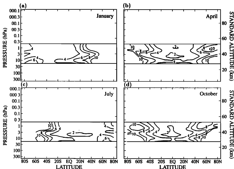
Figure 12. Same as Figure 11, but for 4 years of SBUV results. (Adapted from Keating et al. , 1990, Figure 6, chap. 15 with permission from the Committee on Space Research).
