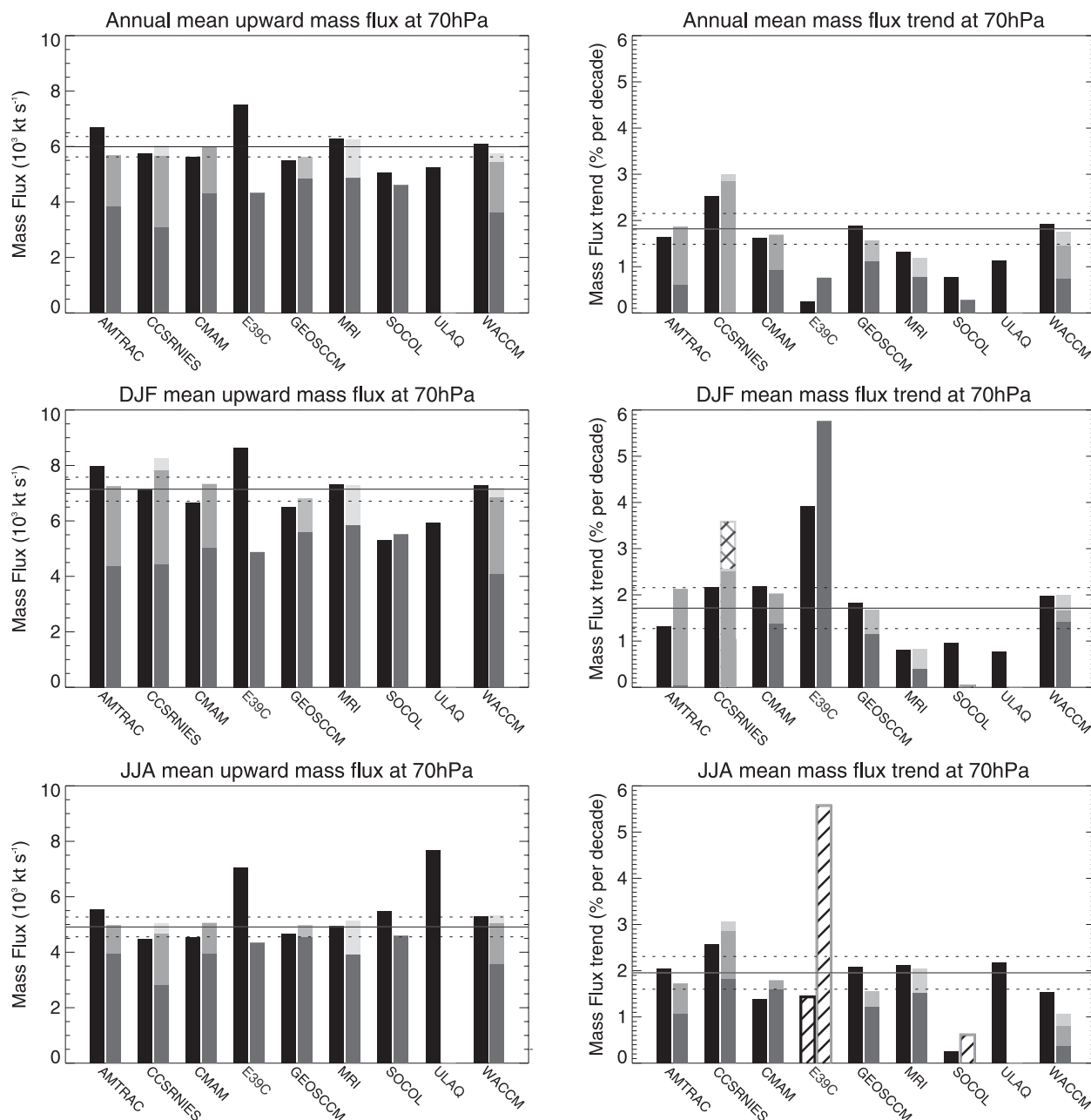
FIG. 11. Comparison of the (top) annual, (middle) December–February, and (bottom) June–August mean tropical upwelling mass fluxes and mass flux trends at 70 hPa (black bars) with those derived from downward control (gray bars). The results are for the total upward mass flux between the turn around latitudes where the residual vertical velocity changes sign from upward to downward. The dark gray shading represents the contribution from the EP flux divergence, with the lighter shadings being the contributions from parameterized orographic and nonorographic gravity waves (lightest shade). The EP flux divergence was not available from ULAQ; GWD was not available for, or not used (see Table 1), in the E39C, SOCOL, and ULAQ models; in addition, nonorographic GWD was unavailable for the AMTRAC. The GWD results shown for the GEOS CCM are the combined orographic and nonorographic contributions. The solid horizontal lines are the multimodel mean with the dashed lines indicating \pm 2 standard error. When results were available for more than one simulation of a particular model the ensemble mean is used in the figure. The diagonal shading indicated negative trends. (left) Mass fluxes for the year 2000 based on a linear fit to the time series. (right) Trends obtained from the linear fit.
